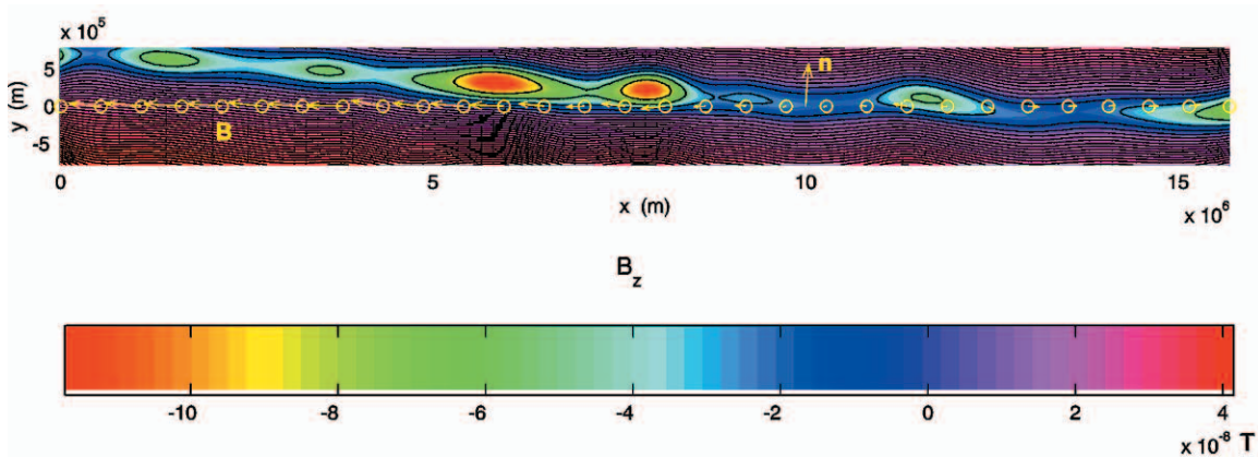
FIGURE 3.10 Magnetic islands along Earth's magnetopause deduced from in situ magnetic field data. These islands have been attributed to the ion-tearing mode. Reprinted, with permission, from L.-N. Hau and B.U.Ö. Sonnerup, Two-dimensional coherent structures in the magnetopause: Recovery of static equilibria from single-spacecraft data, Journal of Geophysical Research 104(A4), 6899-6918, 1999. Copyright 1999, American Geophysical Union.
