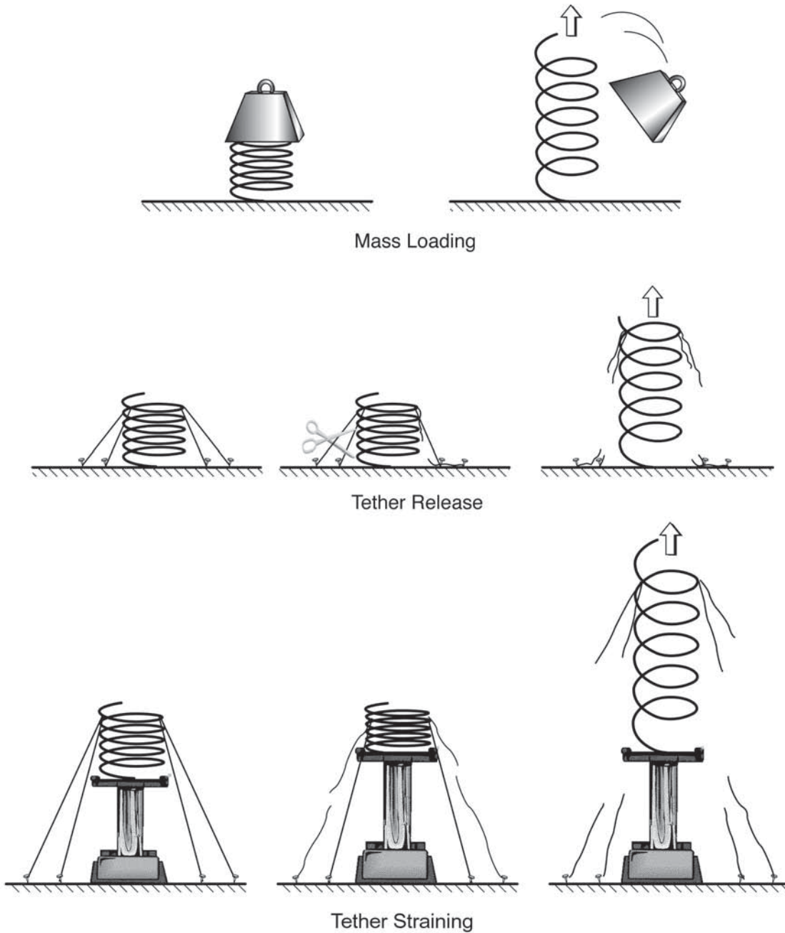
FIGURE 5.2 Three classes of coronal mass ejection models. Image courtesy of J. Klimchuk (Naval Research Laboratory). Reprinted, with permission, from J.A. Klimchuk, Theory of coronal mass ejections , pp. 143-157 in Space Weather , Geophysical Monograph 125, P. Song, H.J. Singer, and G.L. Siscoe, eds., American Geophysical Union, Washington, D.C., 2000. Copyright 2000, American Geophysical Union.
