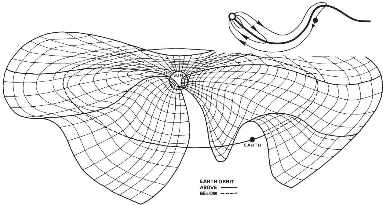
FIGURE 3.6 Schematic diagram of the three-dimensional structure of the current sheet that flows in an azimuthal direction around the Sun. The inset at the top of the figure shows the opposite polarities of the magnetic fields on the two sides of the current sheet. Courtesy of S.-I. Akasofu, Geophysical Institute, University of Alaska.
