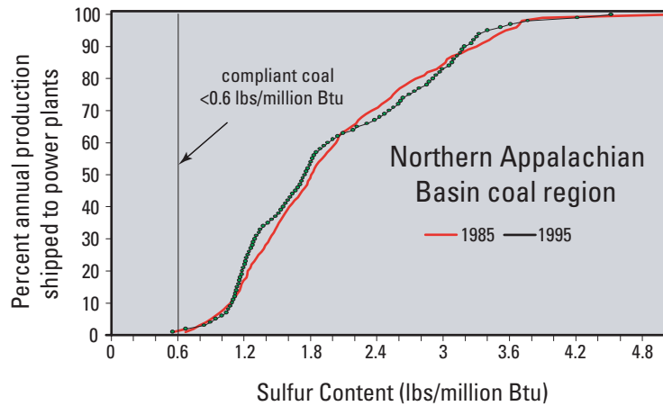
Figure 5. Graphs showing cumulative distribution of U.S. coals shipped to power plants between 1985 and 1995, by pounds of sulfur per million Btu (shown by vertical line in each graph). Phase II of the Clean Air Act Amendments of 1990 (Public Law 101-549) mandates a limit of 0.6 pounds of sulfur per million Btu. About 30 percent of coal from the central
