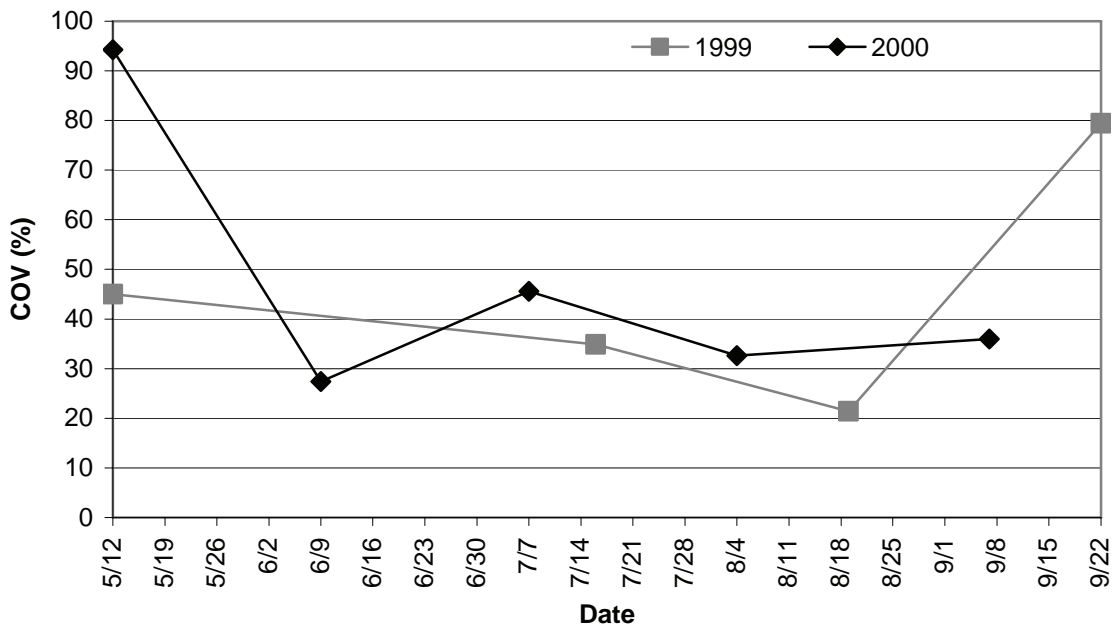
Figure A-20. Coefficient of variation (%) of total number zooplankton ( \# \text{ individuals/m}^2 ) over time for two-yr study.
