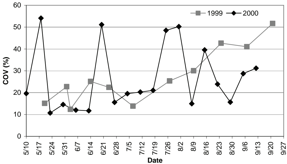
Figure A-4. Coefficient of variation (%) of total phosphorus (µg/L) over time for two-yr study.
