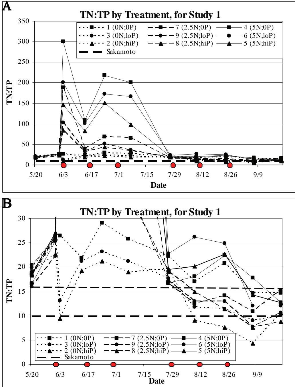
Figure 16. Changes in the ratio of total nitrogen to total by treatment over time. A) TN:TP ratios in all treatments presented with a heavy dashed line representing the range for optimal algal growth proposed by Sakamoto (1966). B) The lower graph is the same as (A), but with the scale enlarged to delineate ratios in the late season. Dark circles on X axis mark dose dates.
