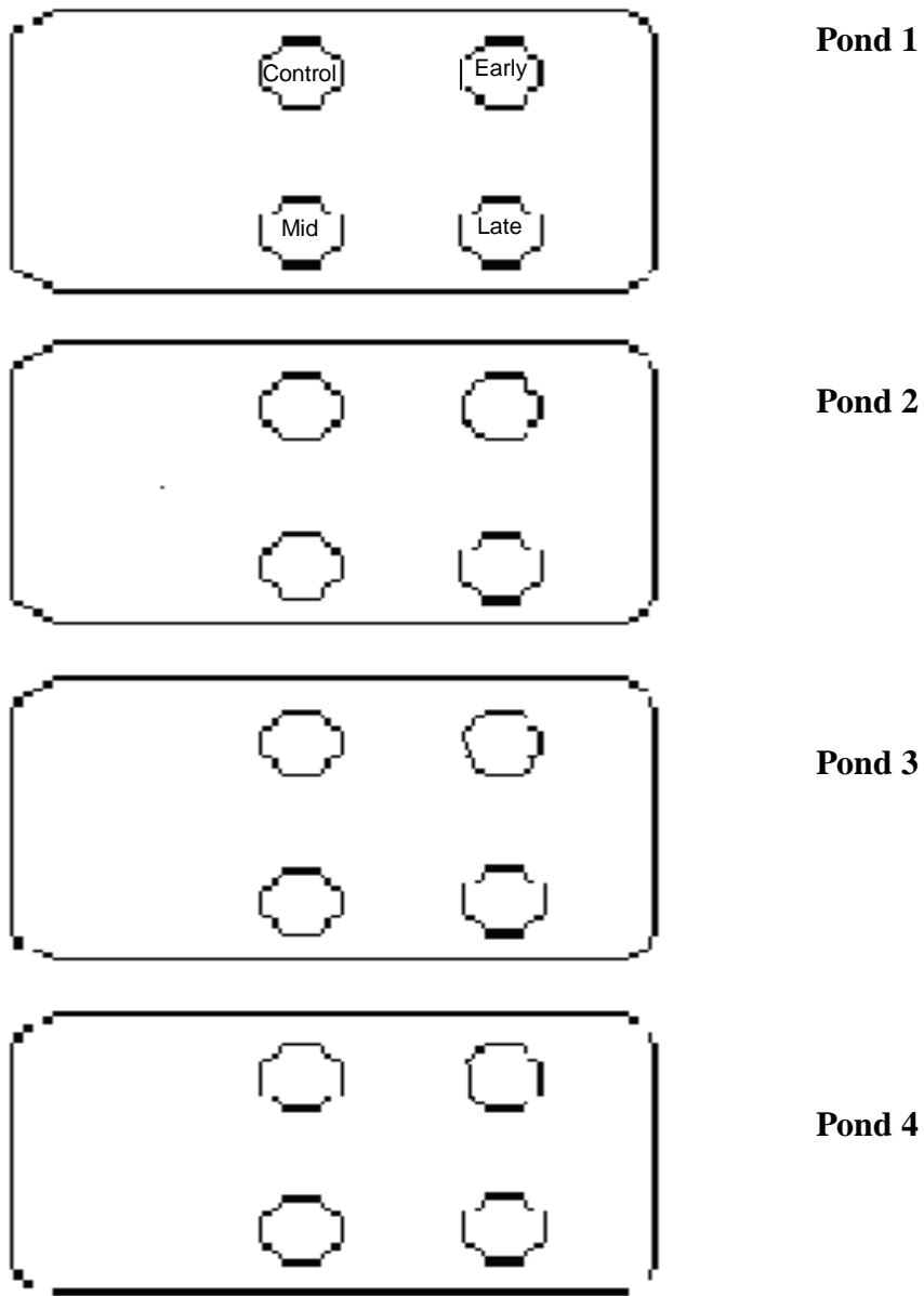
Figure 58. Corral and pond diagram for Study 3 experiments indicating orientation of corrals. Pond 1 shows an example of the random assignment of the treatments.
