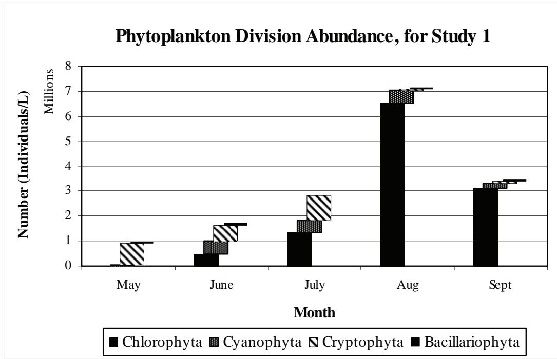
Figure 23. Changes in phytoplankton abundance of the four dominant divisions over time. Columns represent averages of all coralls in each month to show general successional trends over the season.
