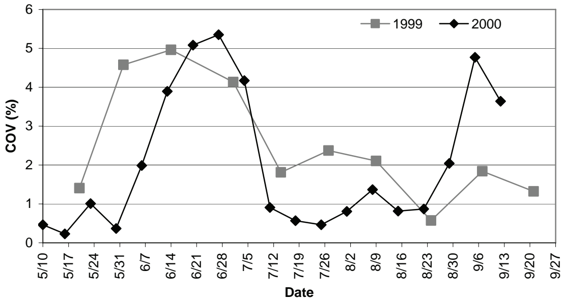
Figure A-8. Coefficient of variation (%) of pH over time for two-yr study.
