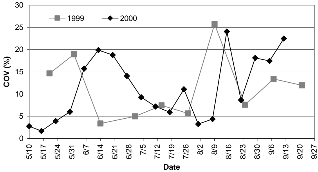
Figure A-9. Coefficient of variation (%) of alkalinity (mg/L) over time for two-yr study.
