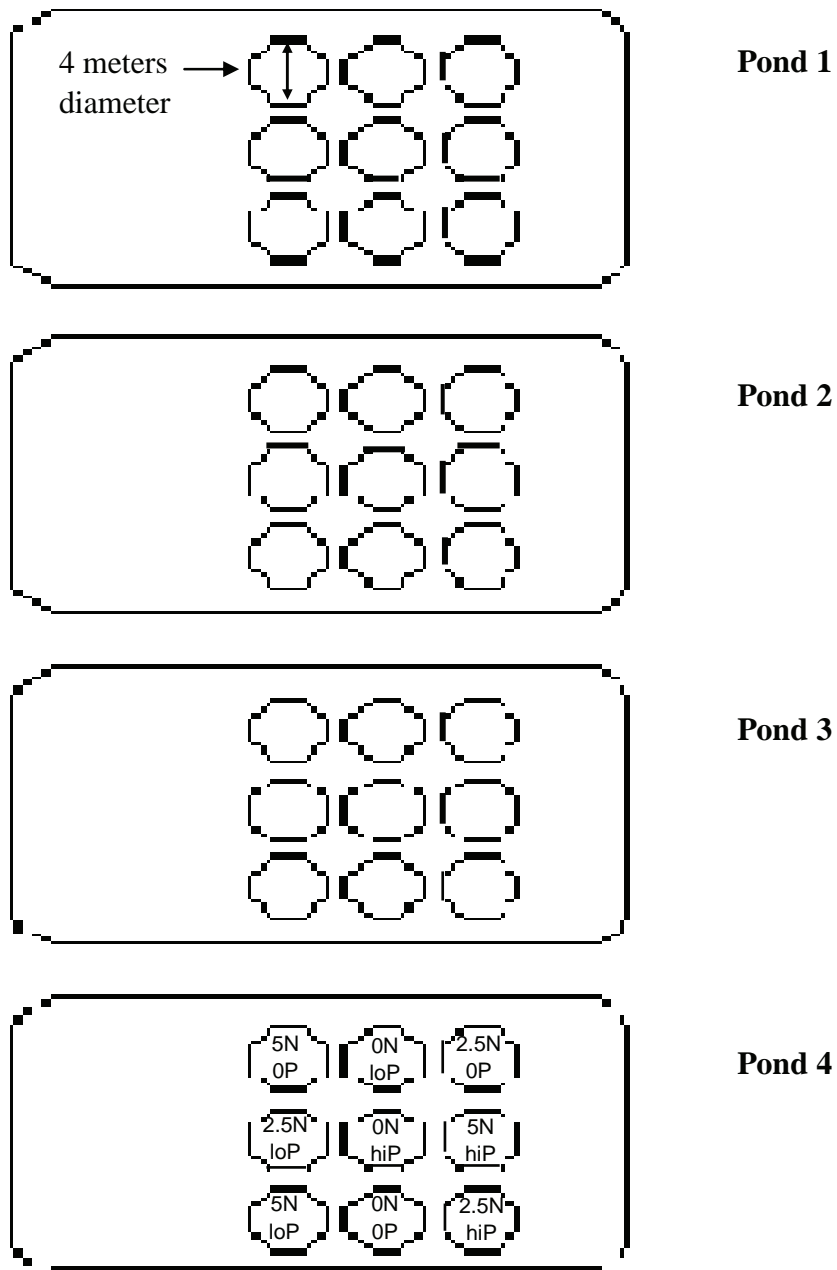
Figure 1. Pond and corral diagram for Study 1 experiments indicating corral orientation and diameter. Pond 4 shows an example of the random assignment of the nine treatments.
