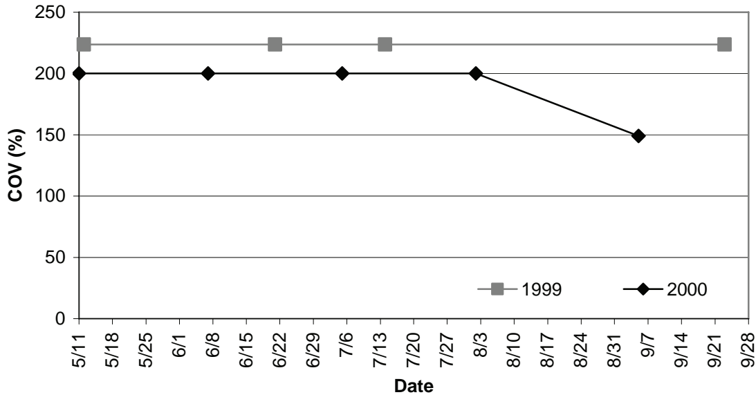
Figure A-42. Coefficient of variation (%) of total numbers euglenophyta (# cells/L) over time for two-yr study.
