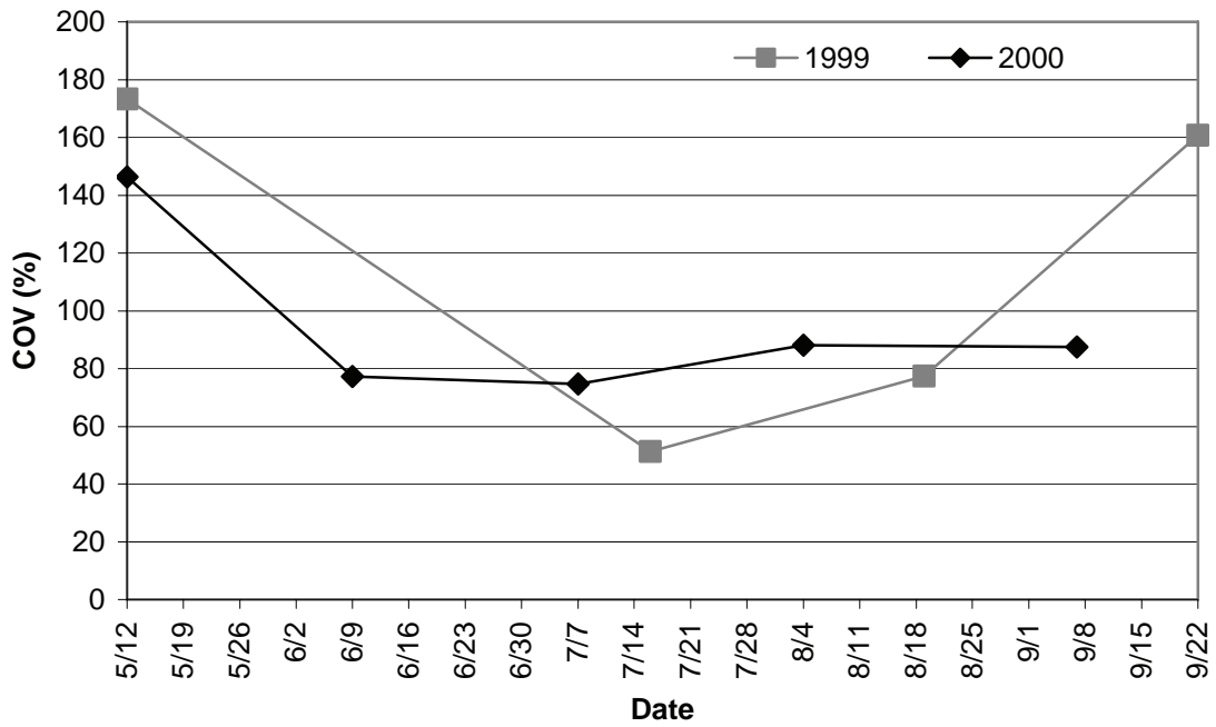
Figure A-29. Coefficient of variation (%) of # individuals of rotifer zooplankton (#/m 2 ) over time for two-yr study.
