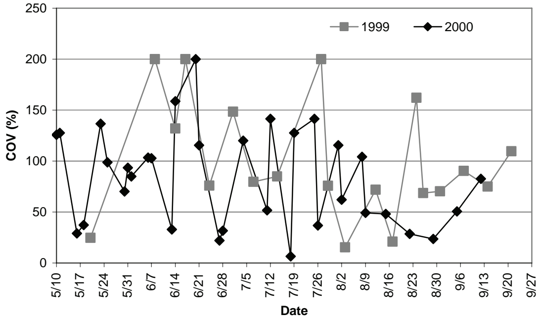
Figure A-5. Coefficient of variation (%) of ammonia (µg/L) over time for two-yr study.
