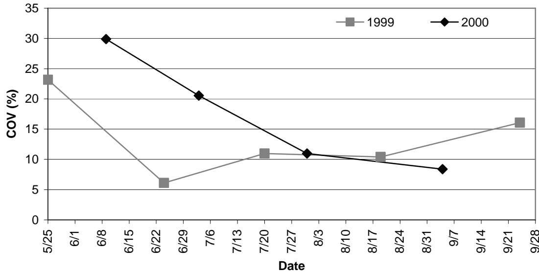
Figure A-16. Coefficient of variation (%) of total nitrogen in macrophytes (% of dry wt.) over time for two-yr study.
