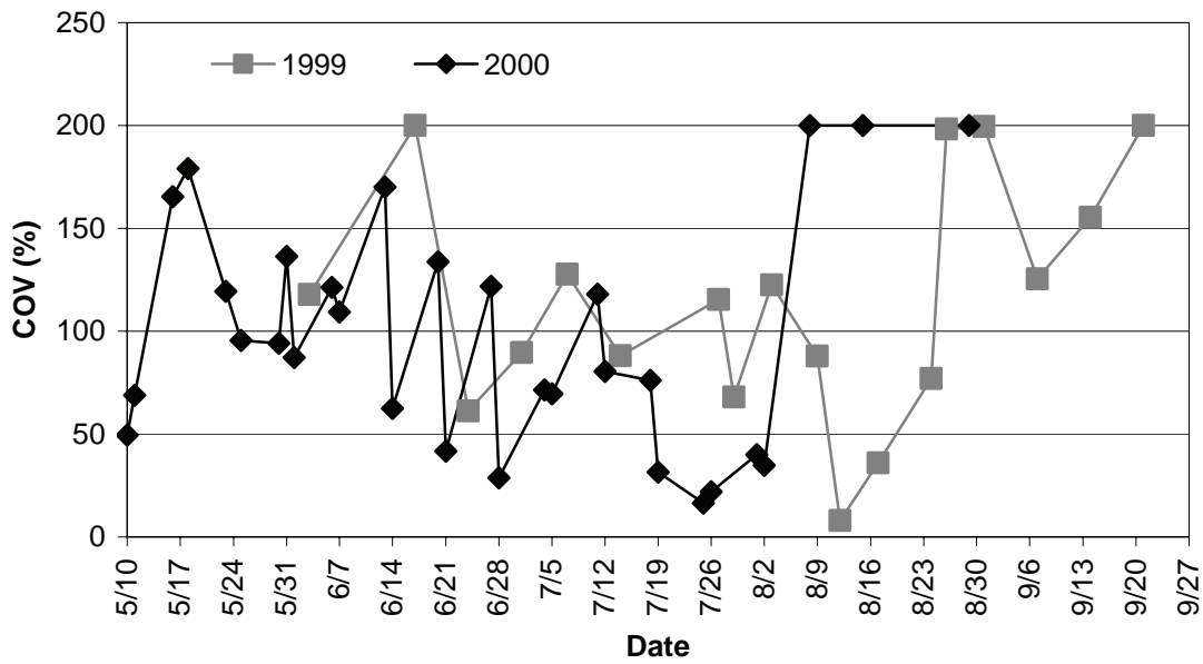
Figure A-6. Coefficient of variation (%) of nitrate / nitrite (µg/L) over time for two-yr study.
