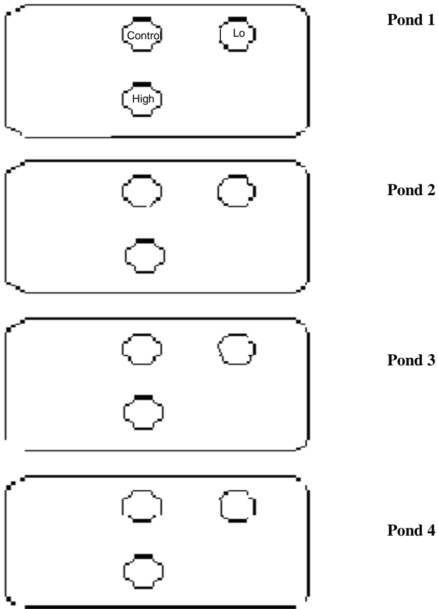
Figure 31. Corral and pond diagram for Study 2 experiments indicating orientation of corrals. Pond 1 shows an example of the random assignment of the treatments.
