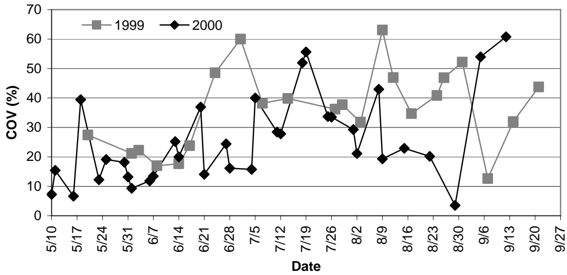
Figure A-7. Coefficient of variation (%) of soluble reactive phosphorus ( \mu\text{g/L} ) over time for two-yr study.
