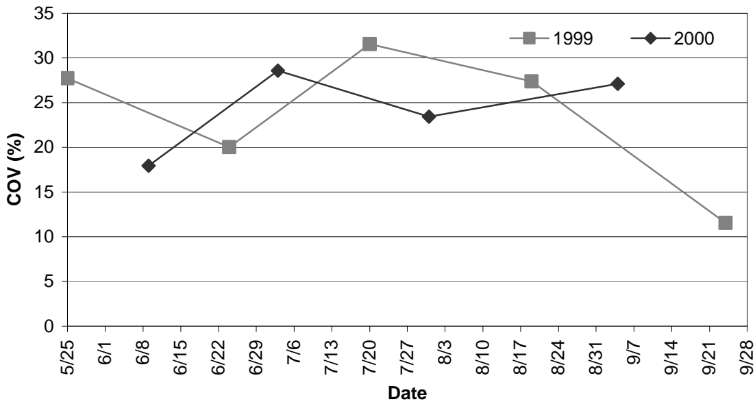
Figure A-18. Coefficient of variation (%) of total nitrogen in sediment ( \text{g N/m}^2 * 5 \text{ cm depth} ) over time for two-yr study.
