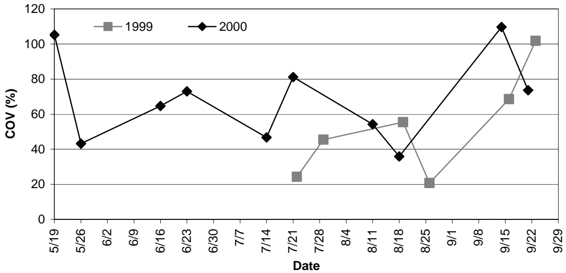
Figure A-2. Coefficient of chlorophyll a in periphyton ( \mu\text{g/cm}^2 ) over time for two-yr study.
