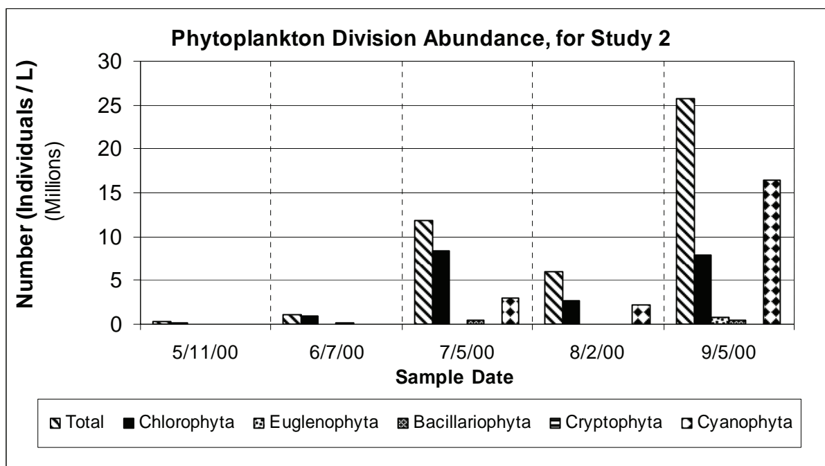
Figure 52. Changes in phytoplankton abundance of the dominant divisions over time. Columns represent averages of all coralls in each month to show general successional trends over the season.
