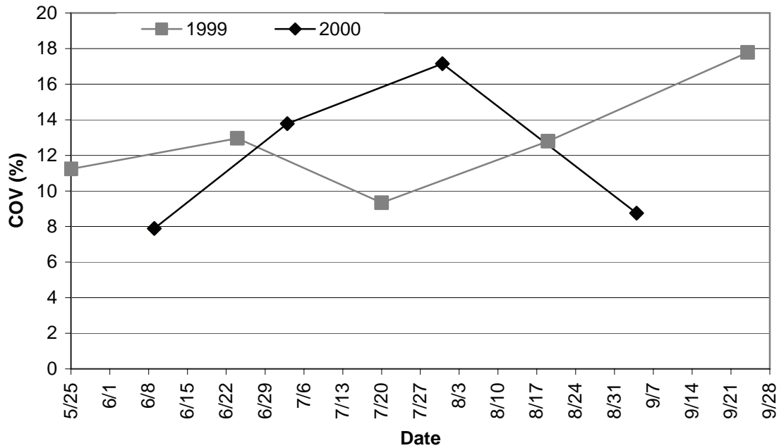
Figure A-19. Coefficient of variation (%) of total phosphorus in sediment ( \text{g P/m}^2 * 5 \text{ cm depth} ) over time for two-yr study.
