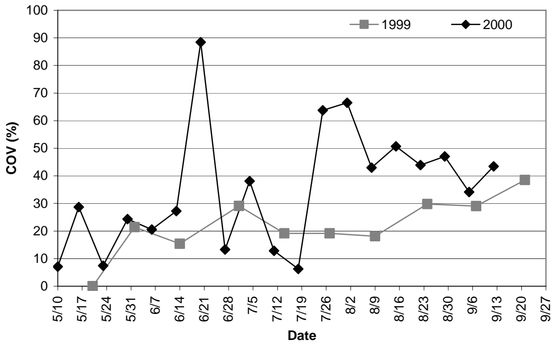
Figure A-12. Coefficient of variation (%) of turbidity (NTU) over time for two-yr study.
