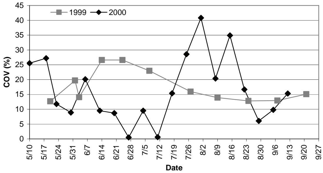
Figure A-3. Coefficient of variation (%) of total nitrogen (mg/L) over time for two-yr study.
