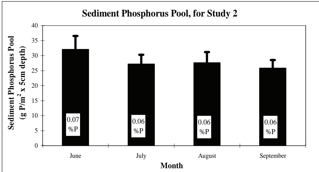
Figure 56. Changes in the sediment phosphorus pool over time. The table presents probabilities that dose, day, and interactions of dose and day influenced P content in sediments in ANOVA of rank-transformed data. Darkened values are not significant ( p > 0.05 ). The graph is a plot of the estimated pool of P in the sediments for an area of 1 m 2 and a depth of 5 cm. Because treatment influences were not significant, monthly values are presented as averages of all treatments. The average %P in sediments is shown within the column for each month.
