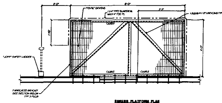
EGRESS PLATFORM PLAN
