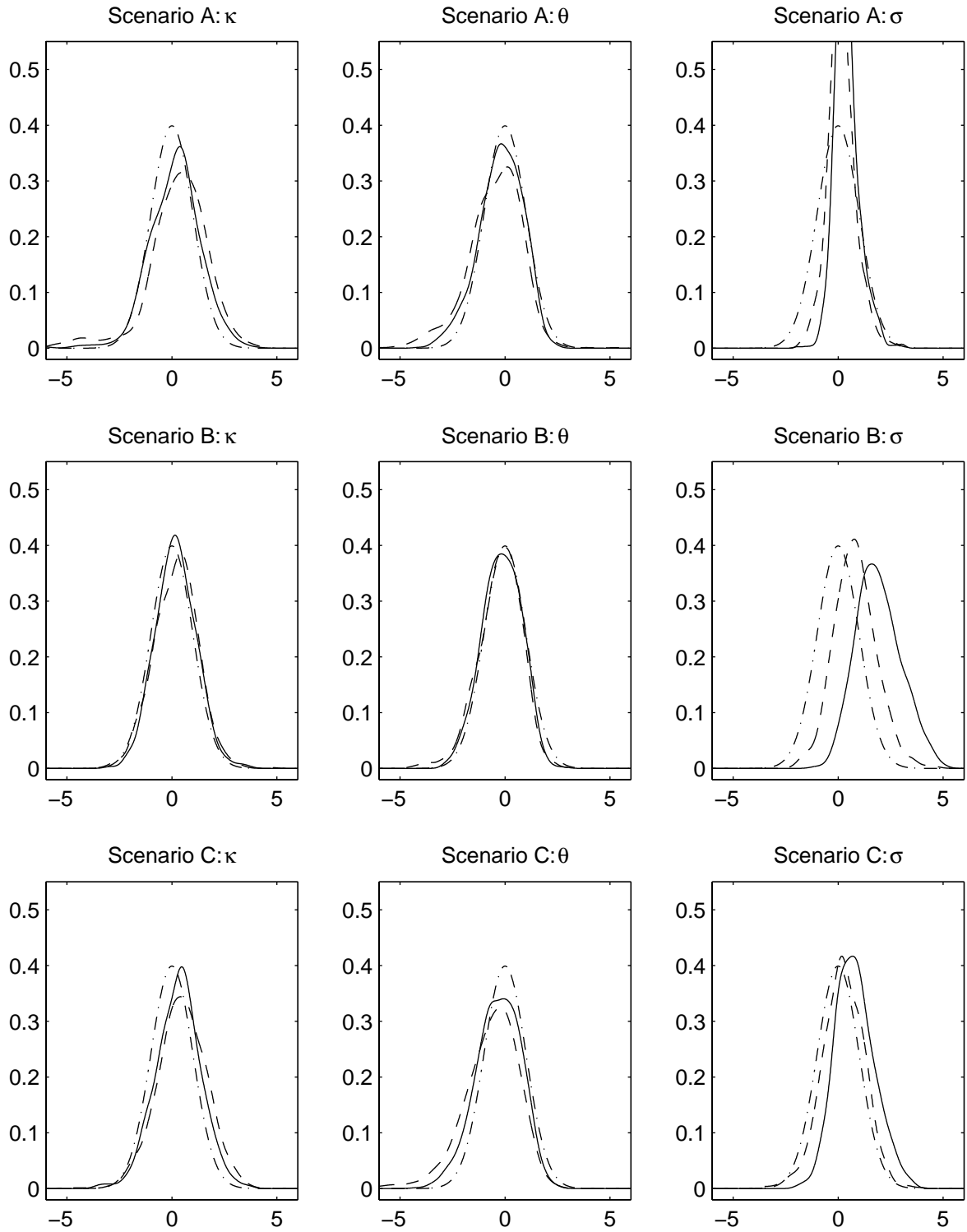
Figure 1: Distributions of t-tests. “- - -” t-statistics with 1,000 observations; “—” t-statistics with 4,000 observations; “-.-” Normal (0,1) reference density.
