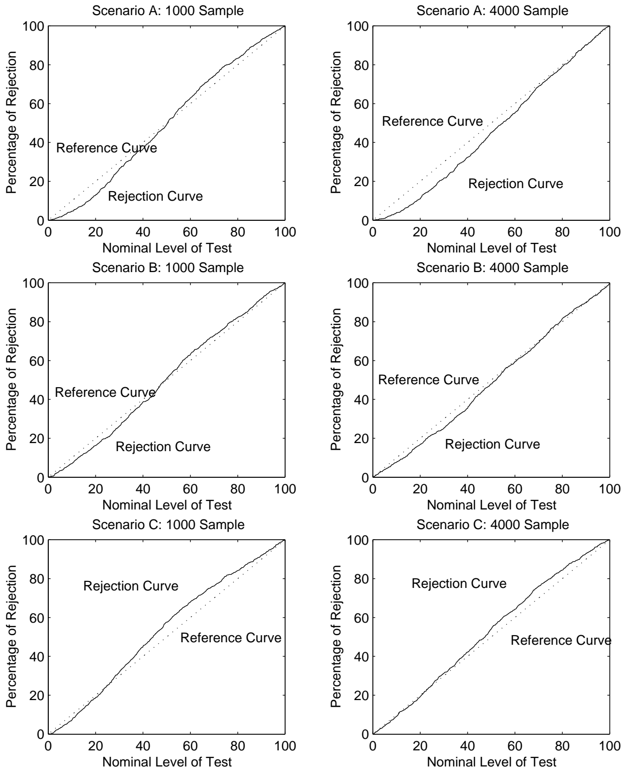
Figure 4: GMM Specification Test of Overidentifying Restrictions with Measurement Error Correction.
