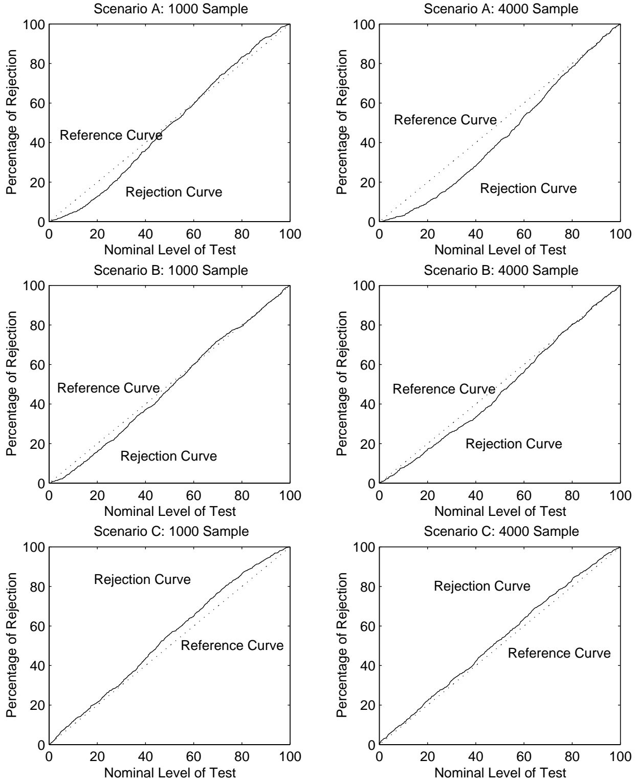
Figure 2: GMM Specification Test of Overidentifying Restrictions.
