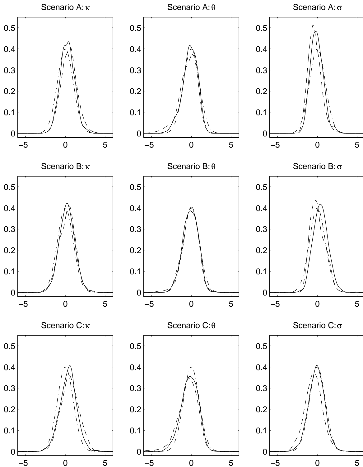
Figure 3: Distributions of t-tests with Measurement Error Correction. “- - -” t-statistics with 1,000 observations; “—” t-statistics with 4,000 observations; “-.-.” Normal (0,1) reference density.
