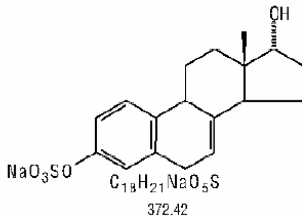
Sodium 17 \alpha -Dihydroequilin Sulfate
