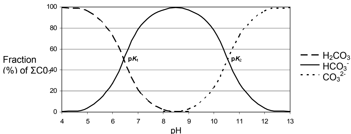
FIGURE 4.—Relation between pH and relative proportions of inorganic carbon species of \text{CO}_2 : ( \text{H}_2\text{CO}_3 ), \text{HCO}_3^- , and \text{CO}_3^{2-} in solution. (modified from Wetzel, 2001).
