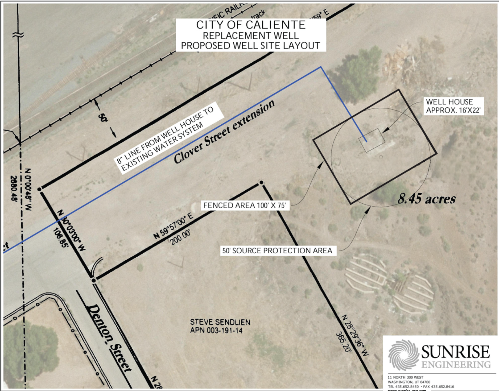
Figure 2 Project Area Caliente Well Replacement Project
