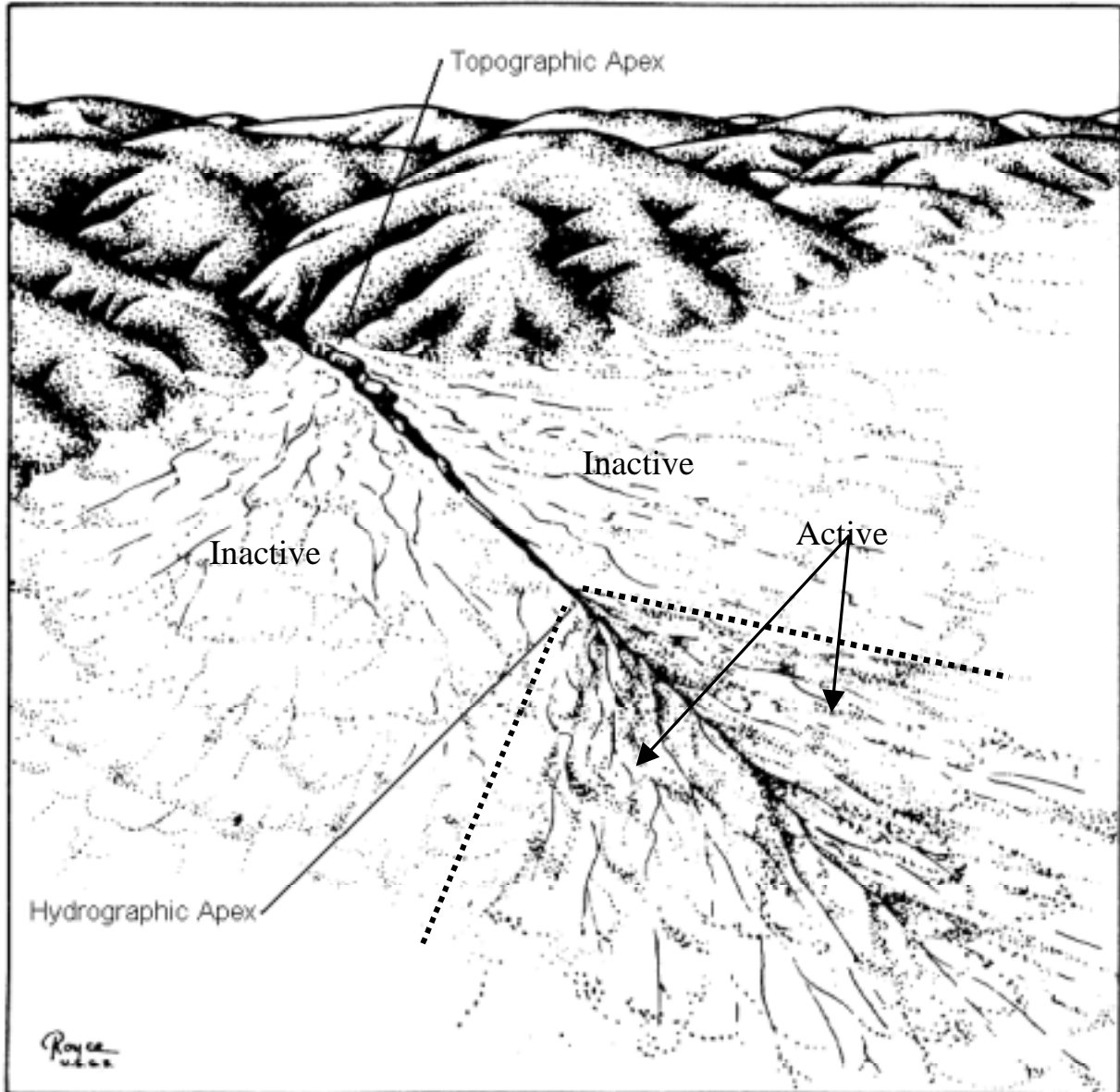
Figure G-1. Alluvial Fan With Entrenched Channel Leading To Active Deposition at Distal Part of the Fan. Original Published as Figure 3-2 in Alluvial Fan Flooding (National Research Council, 1996). Reproduced with Permission From the National Research Council; Annotations Added by FEMA.
