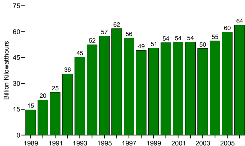
Energy Savings, 1989-2006
