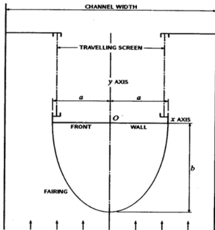
Figure 4. Top view of an elliptical fairing for a dual flow intake screen. Arrows show the direction of flow before turning into screen face. From Fletcher (1994).
