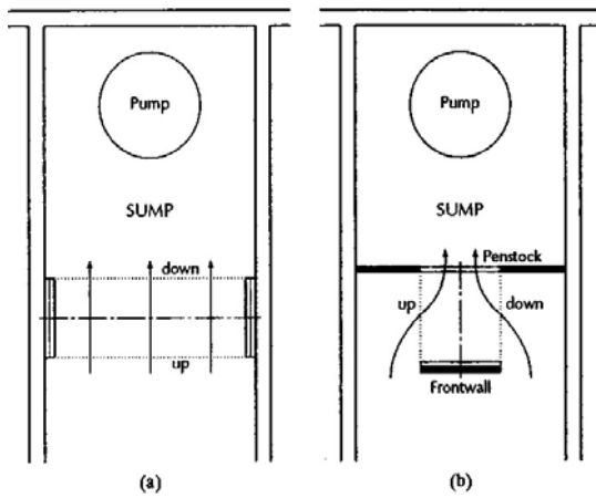
Figure 2. Plan of intake channel equipped with a through flow screen (a) and dual flow screen (b). From Fletcher (1994).
