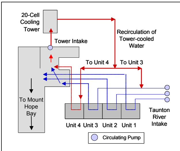
Figure 6. EMM—Unit 4 “Closed Cycle” and Unit 3 “Partial Closed Cycle”
