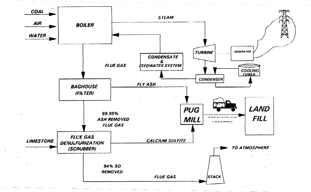
Facility A Process Diagram and CCR Sampling Location
