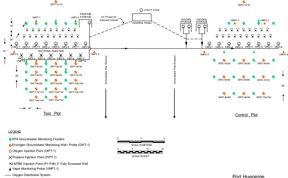
Port Huene EPA MTBE Performance Monitoring In-Situ Biostimulation Bioaugmentation Area Layout
