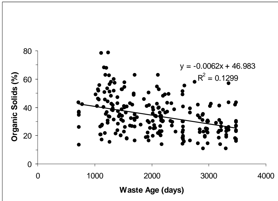
Figure B-2 Relationship between Organic Solids and Waste Age in the Retrofit cell
