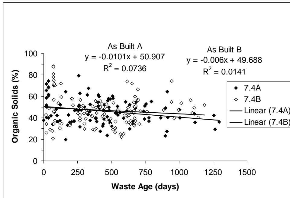
Figure B-10 Relationship between Organic Solids and Waste Age in As-Built cells A and B
