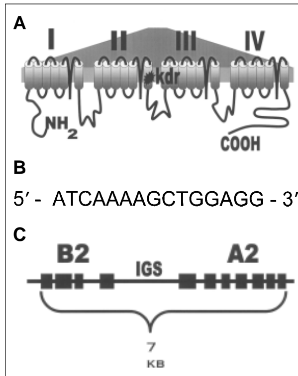
Figure 1. Examples (drawn from references cited in the text) of biochemical resistance mechanisms on the molecular level. A. Single amino acid mutation in the IIS6 membrane-spanning region of the sodium channel gene that confers target-site DDT-pyrethroid resistance in Anopheles gambiae . The same mutated codon produces resistance in insects as diverse as mosquitoes, cockroaches, and flies. B. Regulatory element (found upstream of coding sequence) termed the “Barbie Box” that allows induction of insecticide detoxifying oxidase and esterase resistance genes. Many such putative control elements have been found associated with vector resistance enzymes. C. Esterase A2-B2 amplicon. These resistance esterase genes lie 5' end to 5' end within the same amplification unit. More than 100 copies of this amplicon may be present in a single mosquito. This is one example of a family of amplified esterase genes.
