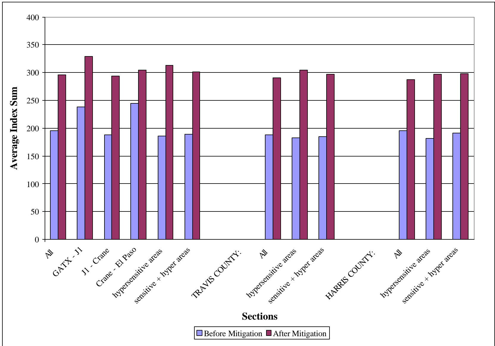
Figure 9-6. Pipeline Segment Averages Before and After Mitigation
