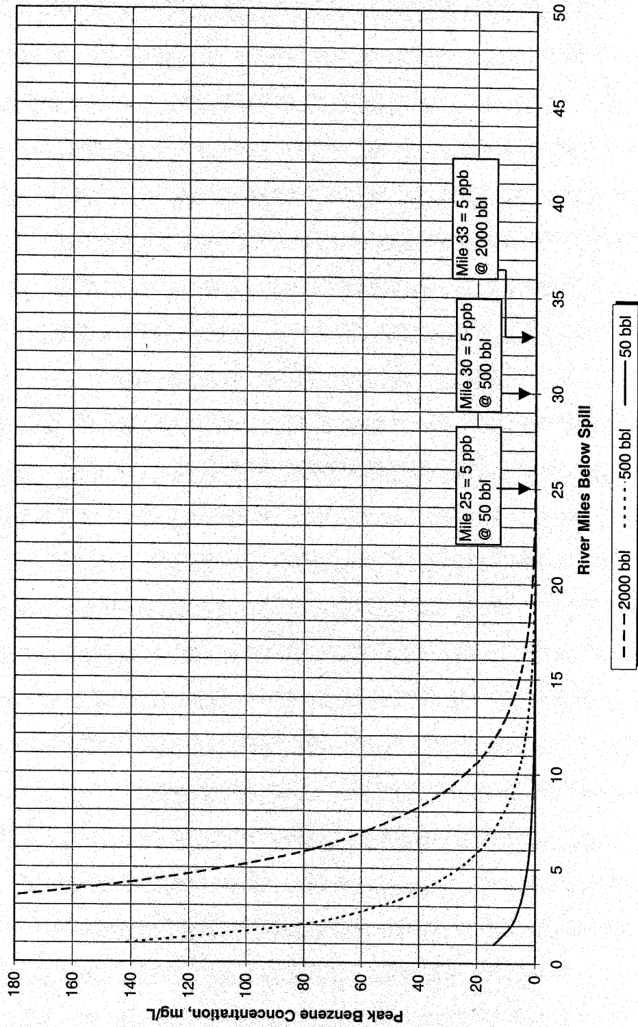
Figure 5-3 Gasoline Spills, 200 cfs, Colorado River
