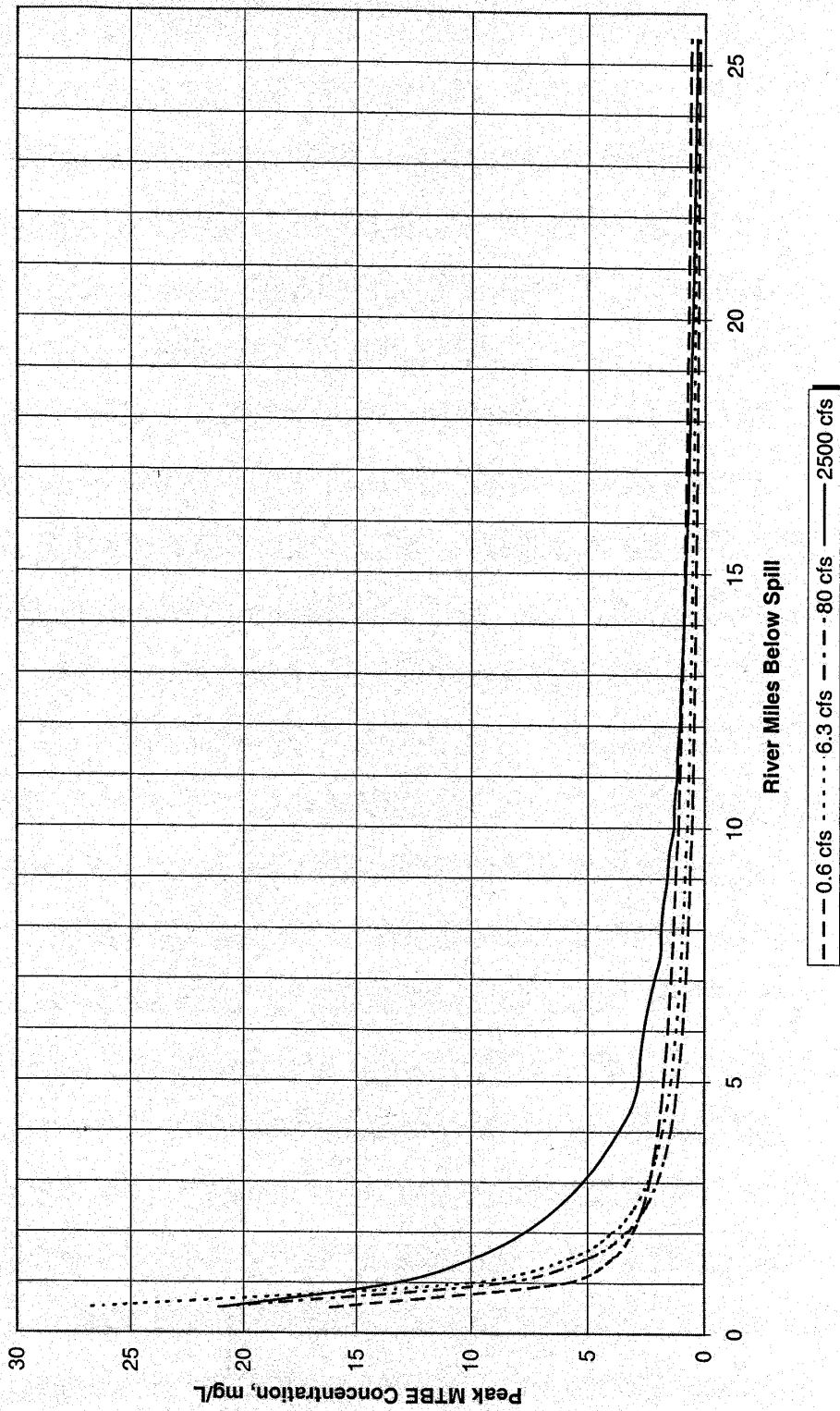
Figure 5-9 50-bbl Gasoline Spill (15% MTBE), Onion Creek
