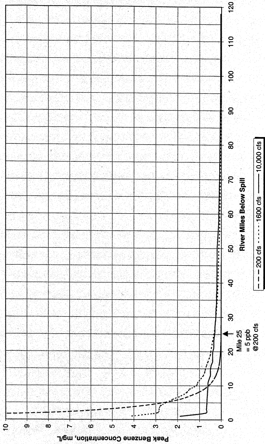
Figure 5-2 50-bbl Gasoline Spill (4.9% Benzene), Colorado River
