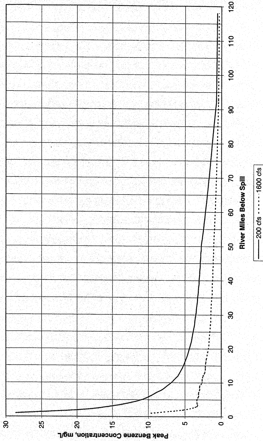
Figure 5-4 85,100-gallon Crude Oil Spill (0.14% Benzene), Colorado River
