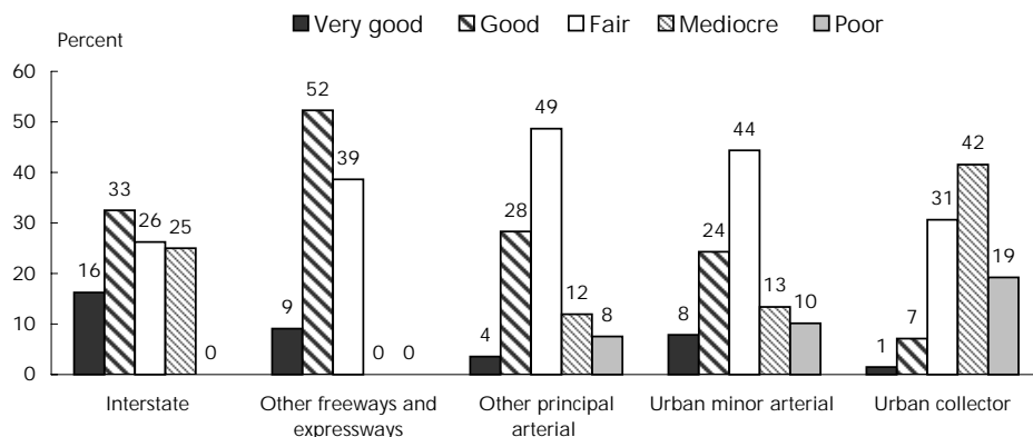
Figure 1-2: Urban Road Conditions in Nevada: 2000
