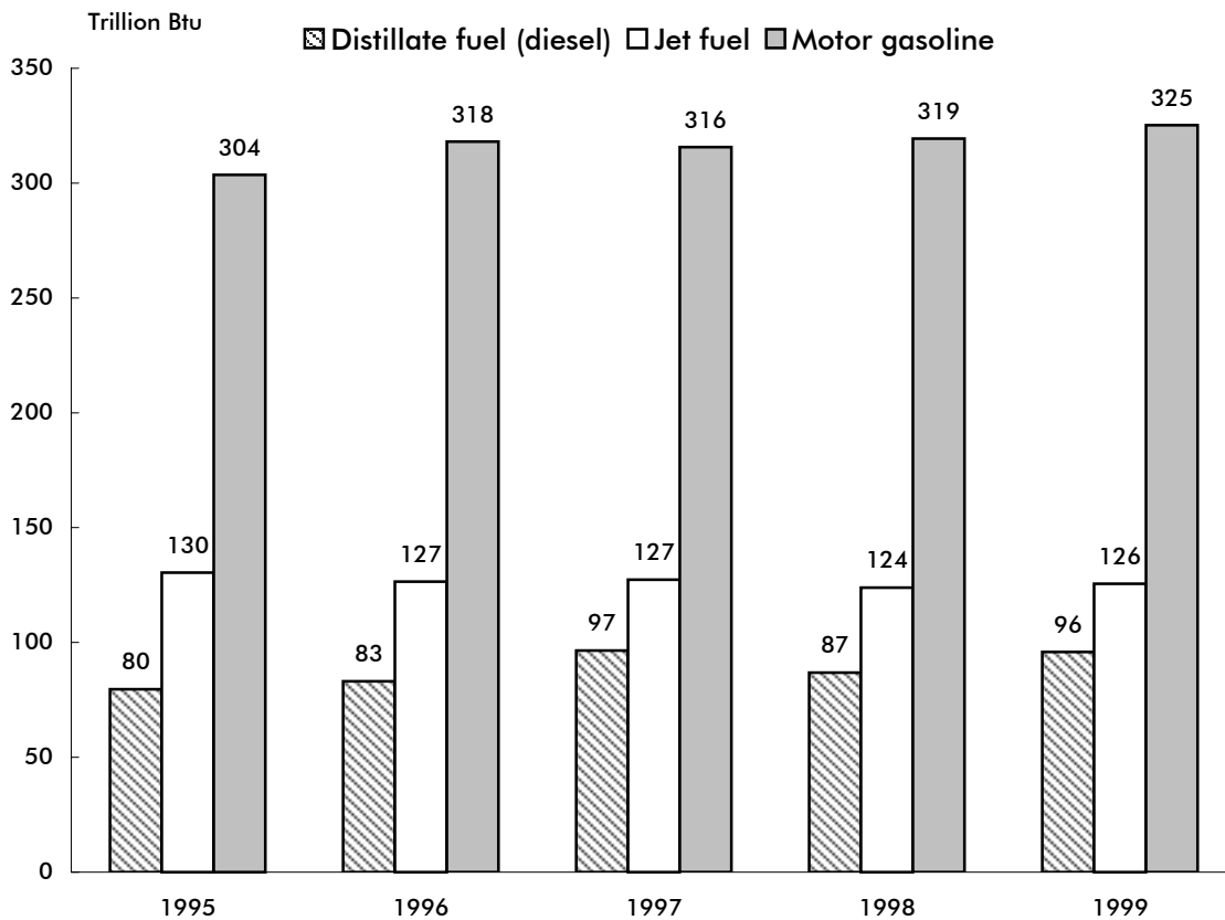
Figure 7-2: Washington Transportation Energy Consumption
