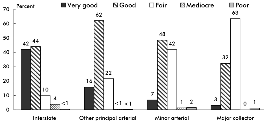
Figure 1-1: Rural Road Conditions in Washington: 2000
