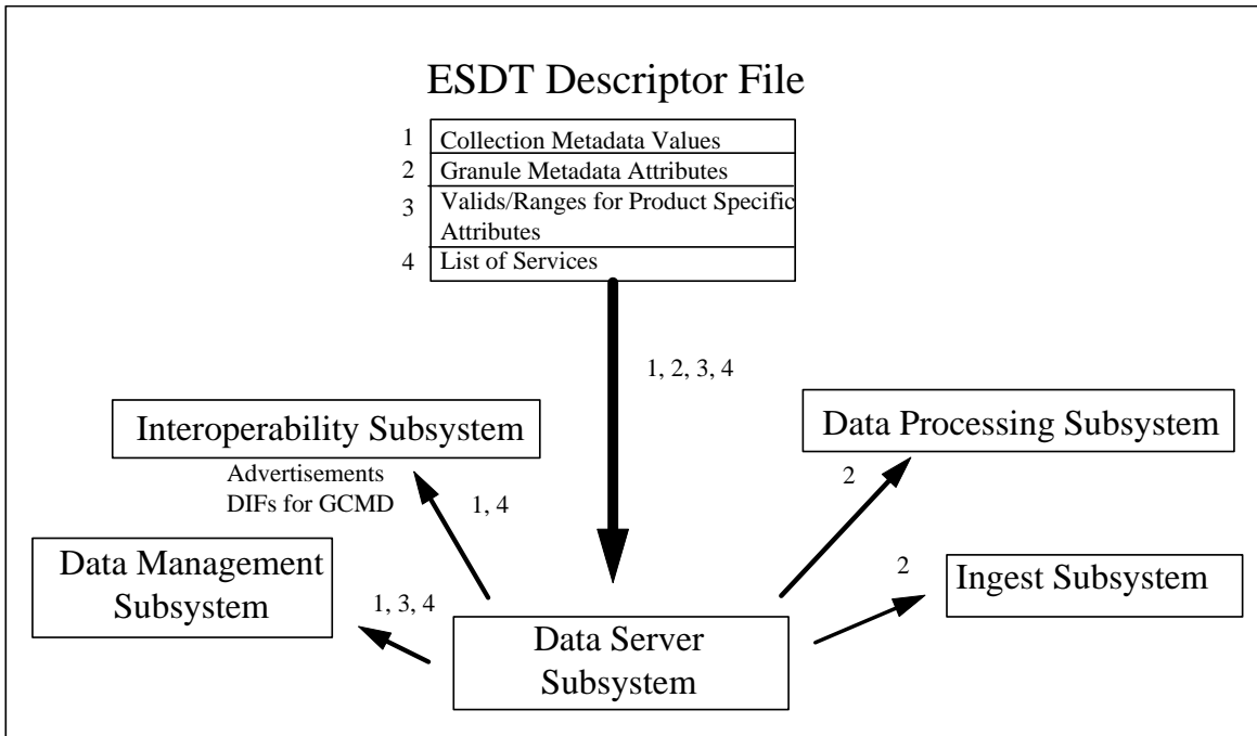
Figure D-1. Metadata Flow in ECS
