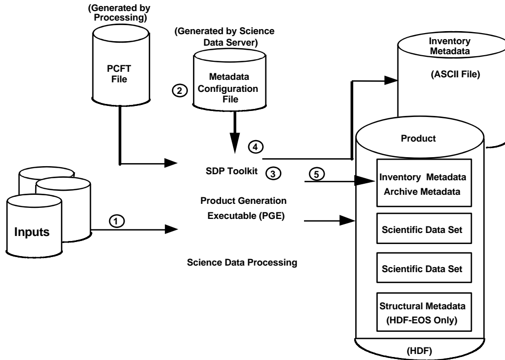
Figure D-5. Science Data Production and Archival Scenario.
