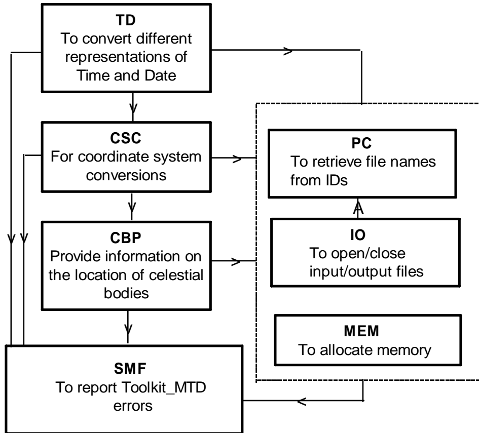
Figure 3-2. Diagram Showing the Relation Between TD Tools and Support Tools
