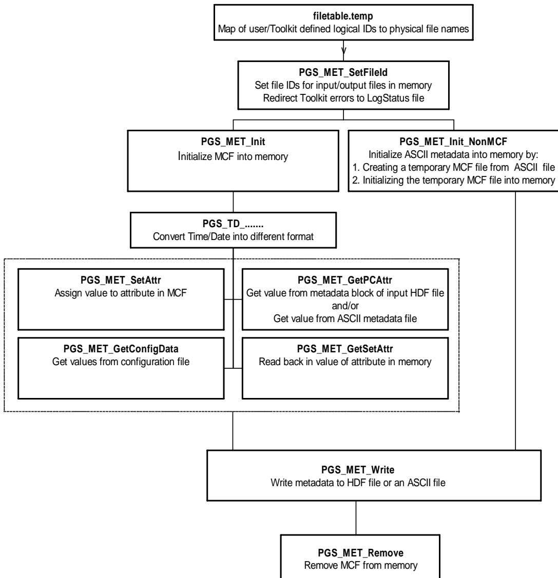
Figure 3-3. Data Flow Diagram
