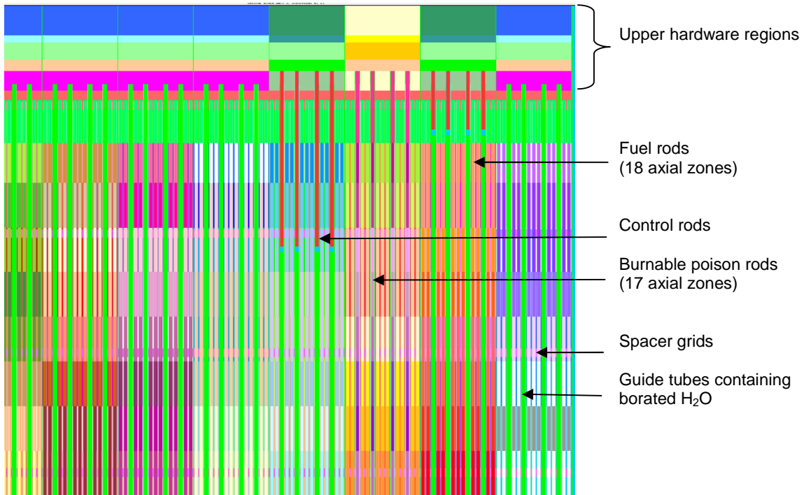
Fig. 7. Horizontal and partial vertical cross sections of KENO V.a geometry for a Crystal River Unit 3 state-point.
