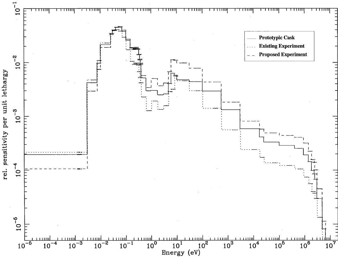
Figure 2. ^{235}\text{U} Capture Sensitivity Profiles for Prototypic Cask, Sample Existing Critical Experiment and a Typical Proposed Critical Experiment
