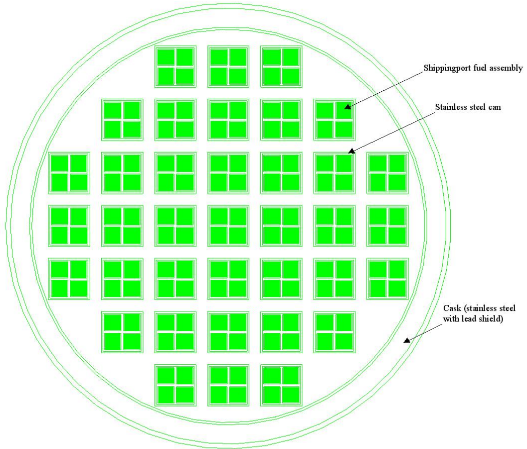
Figure 1. Cross-Section View of Shippingport PWR Fuel Elements in Shipping Cask
