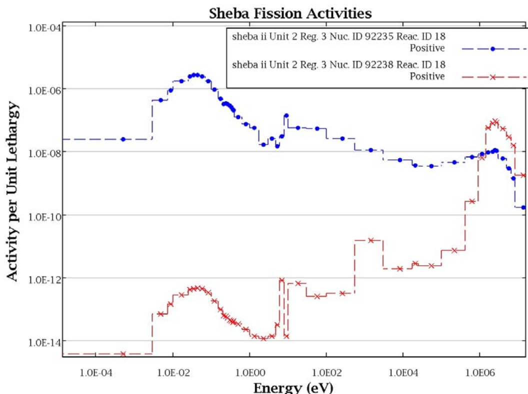
Figure 5. Javapeño plot of ^{235}\text{U} and ^{238}\text{U} fission activities.
