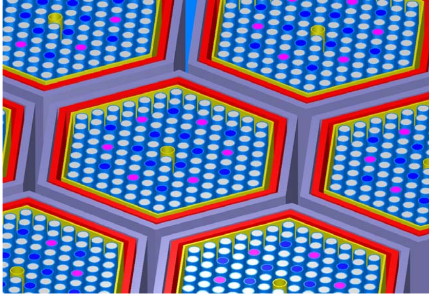
Figure 3. KENO3D close-up view of assemblies in cask.
