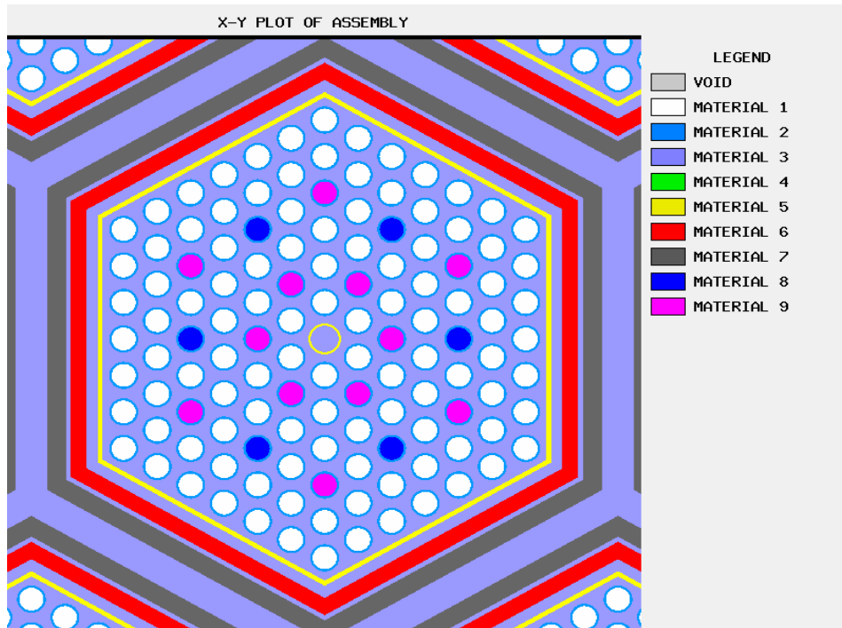
Figure 2. Sample 2-D KENO-VI geometry plot.
