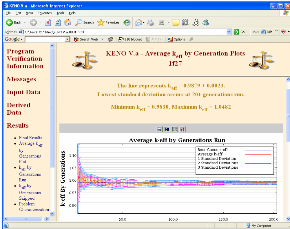
Figure 6. Plot of average k_{eff} by generations run.
