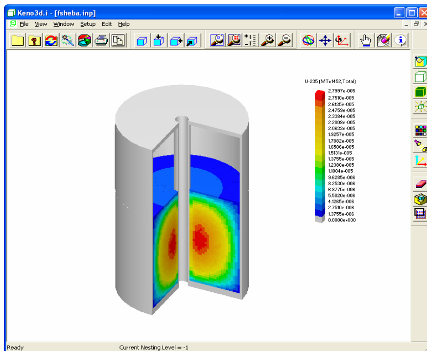
Figure 4. KENO3D plot of the ^{235}\text{U} fission activity.
