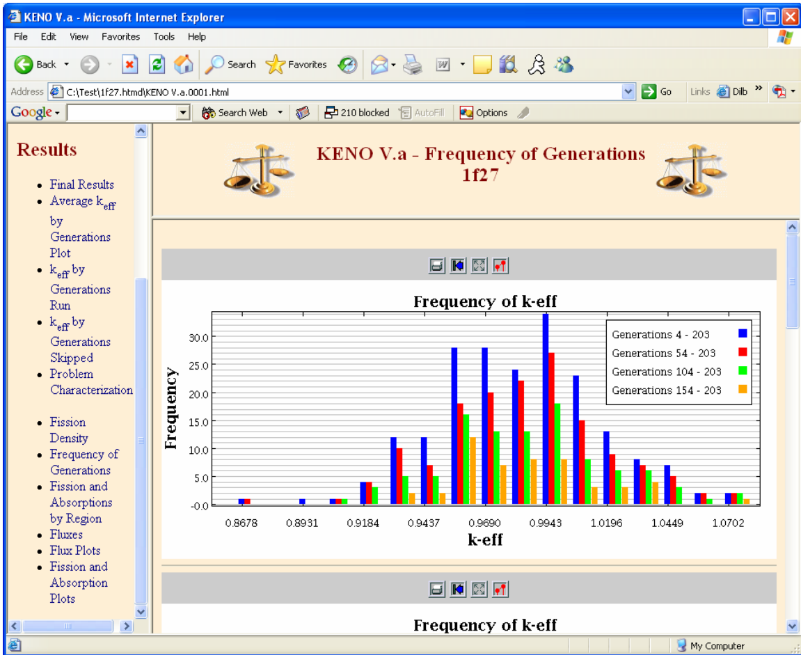
Figure 8. Plot of frequency of k_{eff}
