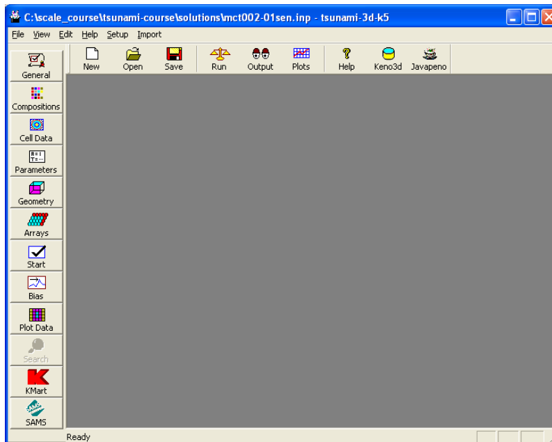
Figure 1. GeeWiz toolbars
