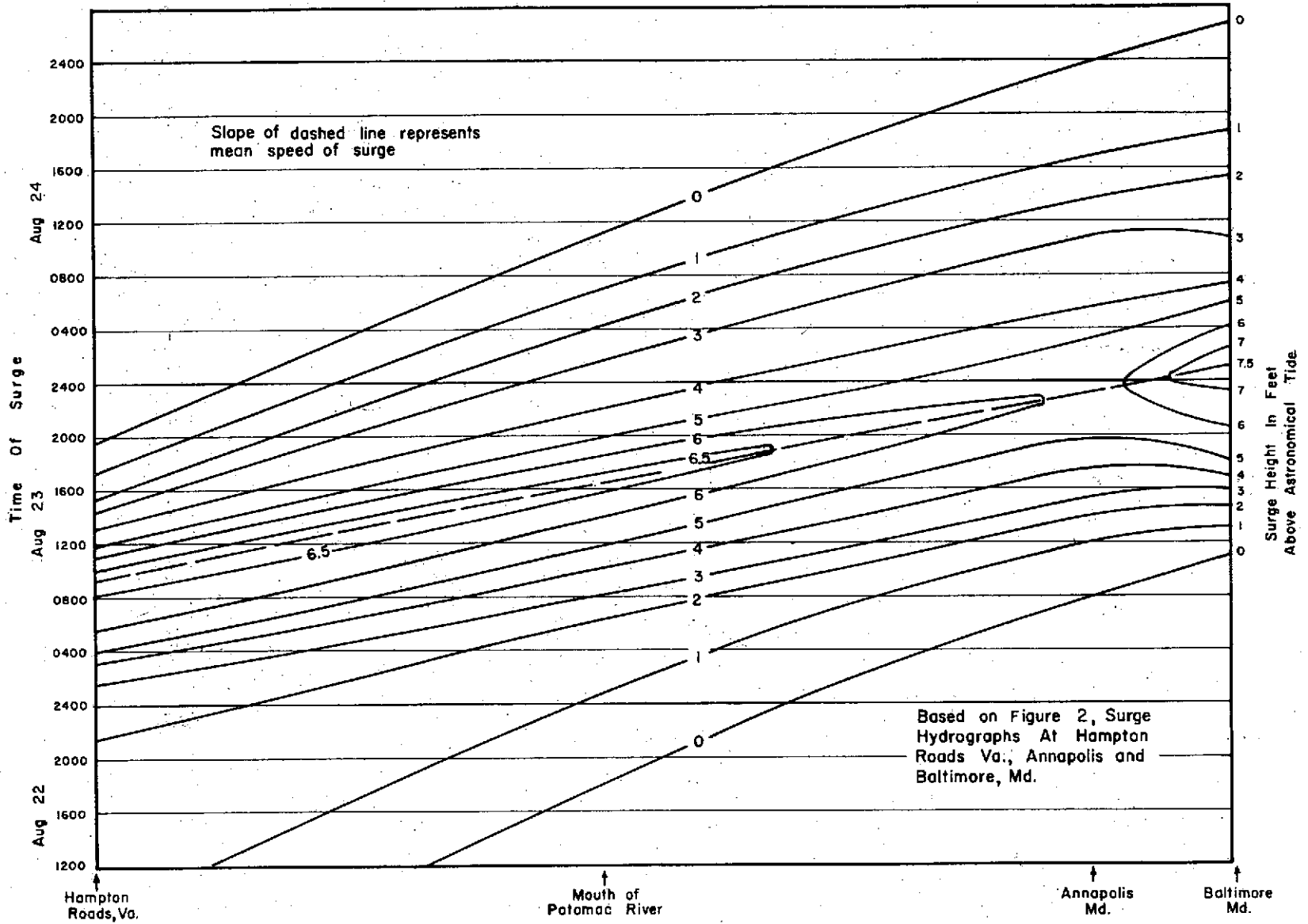
FIGURE 6. ISOLINES OF SURGE HEIGHT VERSUS TIME AND POSITION OF OCCURRENCE (1933 HURRICANE).
