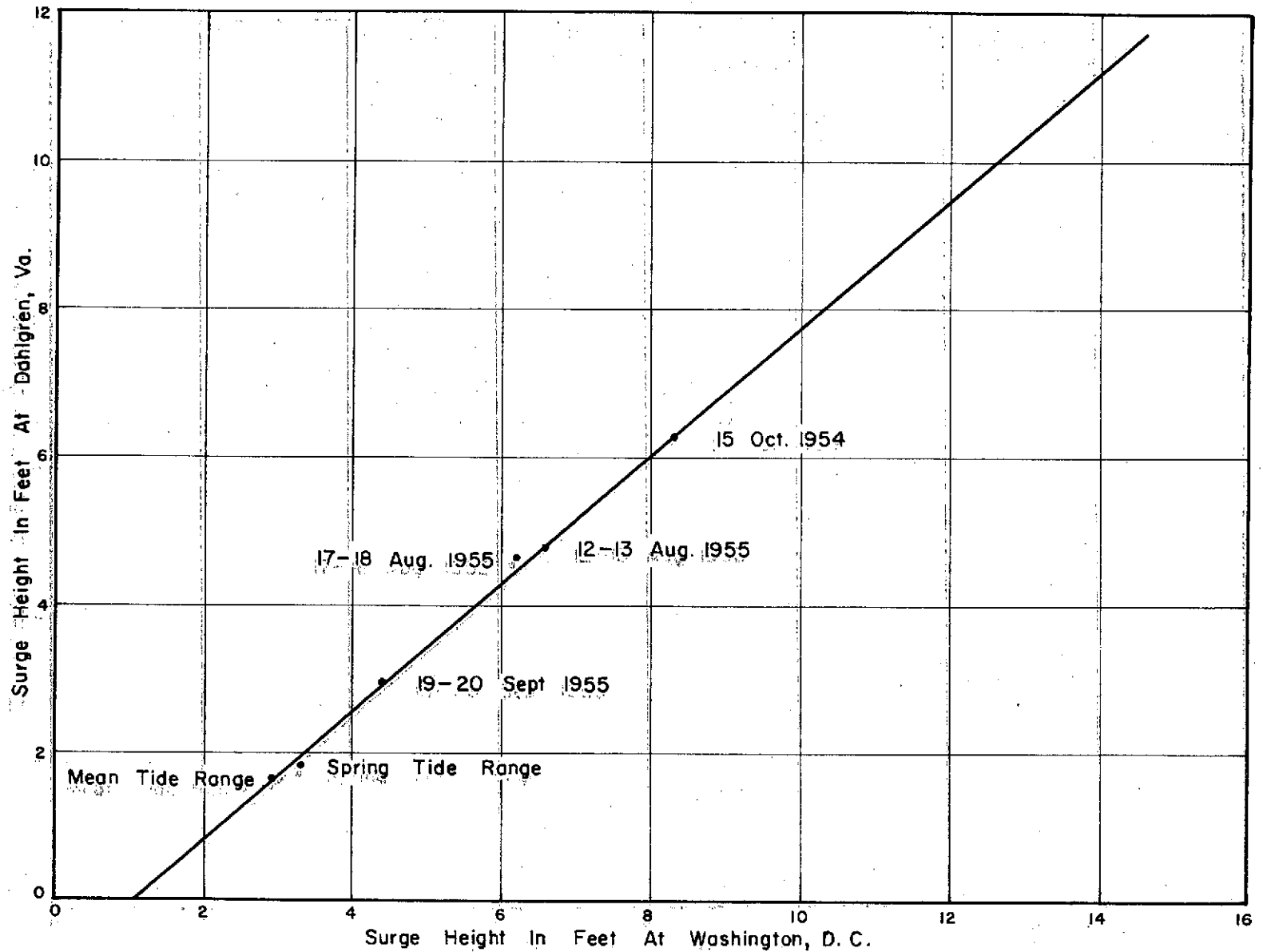
FIGURE 19. SURGE HEIGHT AT DAHLGREN, VA. VS SURGE HEIGHT AT WASHINGTON, D.C.
