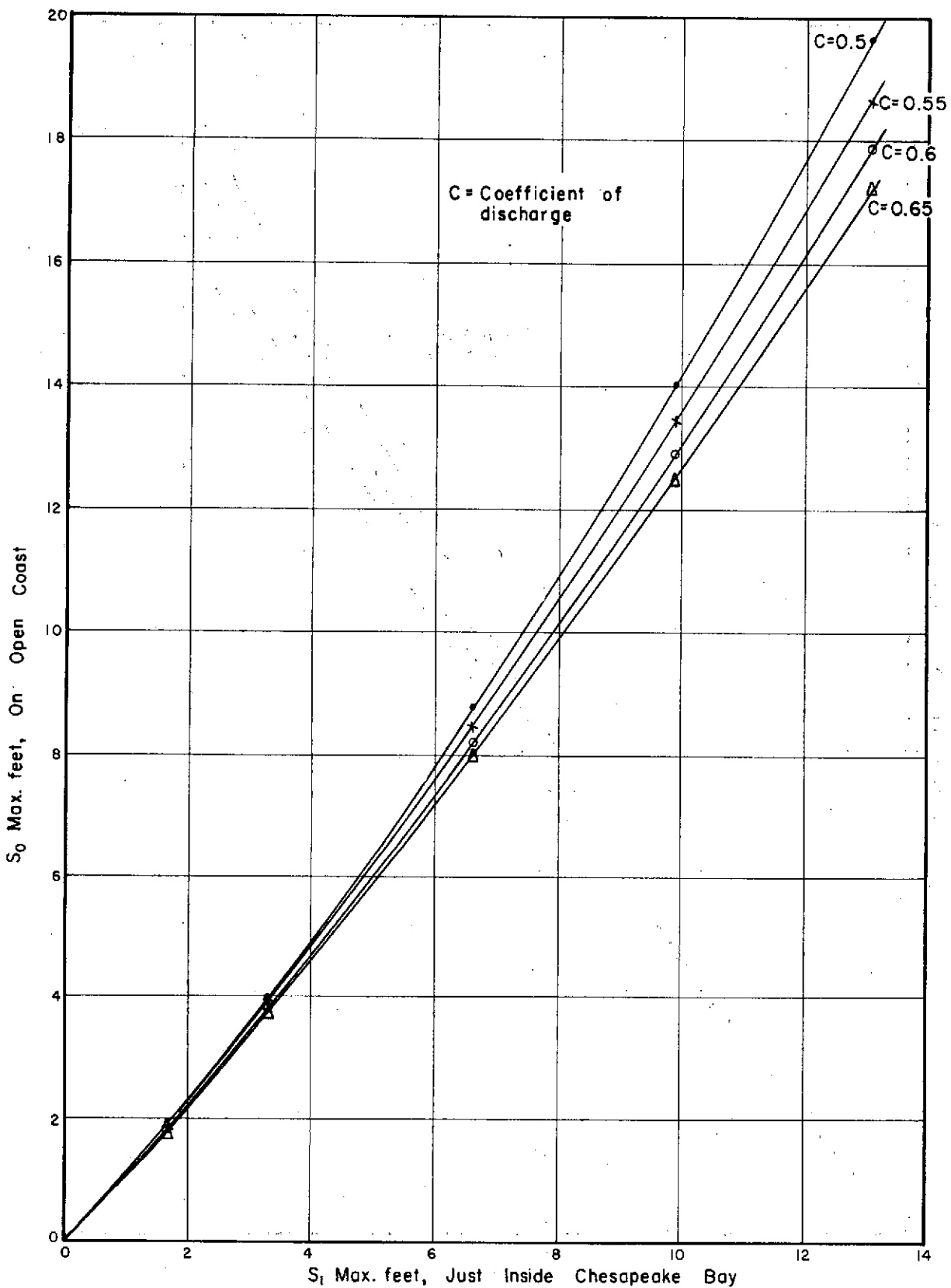
FIGURE 14. PEAK OF SURGE HYDROGRAPH ON OPEN COAST VERSUS PEAK OF SURGE HYDROGRAPH JUST INSIDE CHESAPEAKE BAY. FOR A_u = 80,000 (30 + h_0)
