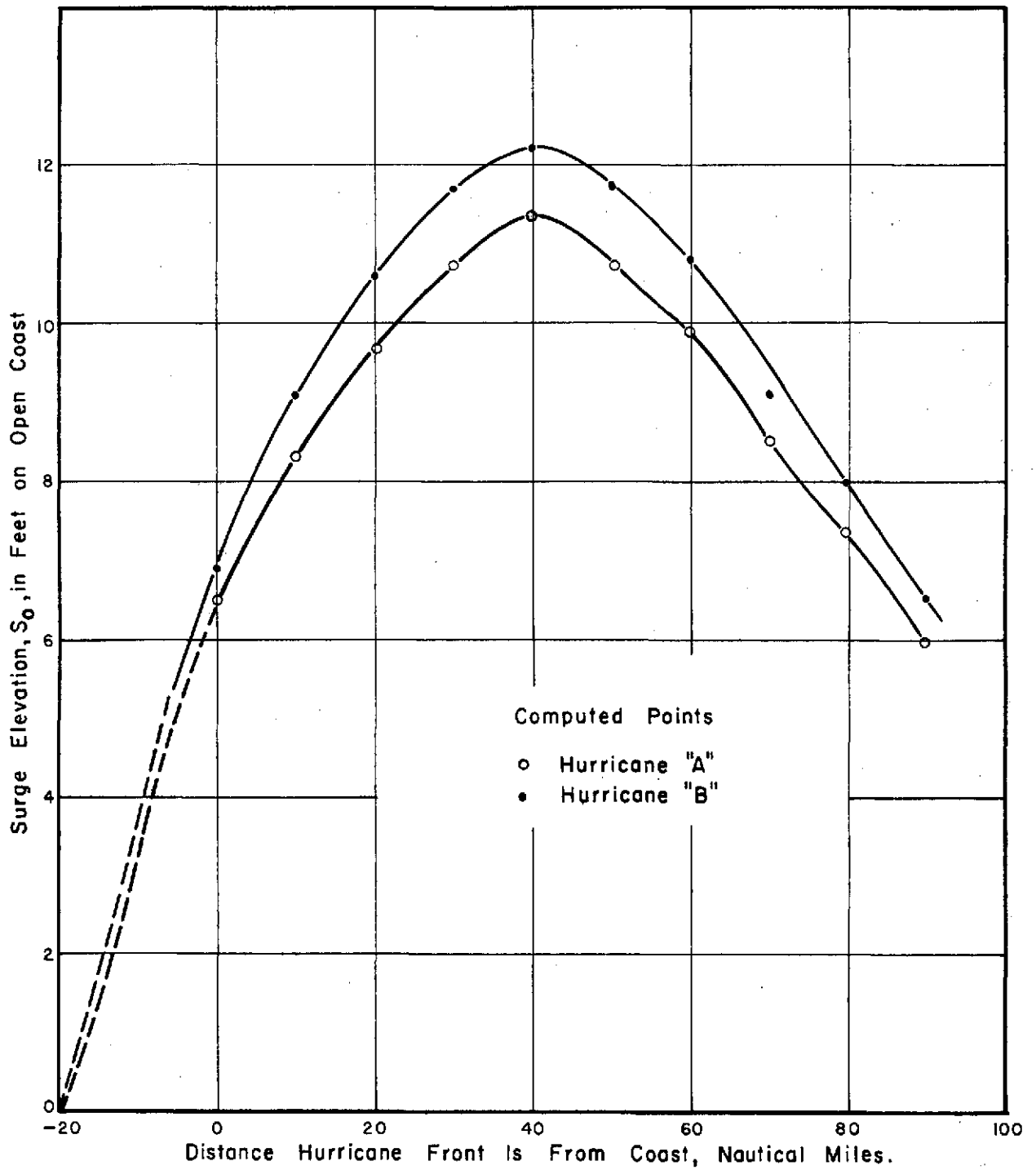
FIGURE 18. SURGE ELEVATION ON OPEN COAST CHESAPEAKE BAY ENTRANCE FOR HURRICANES "A" AND "B".
