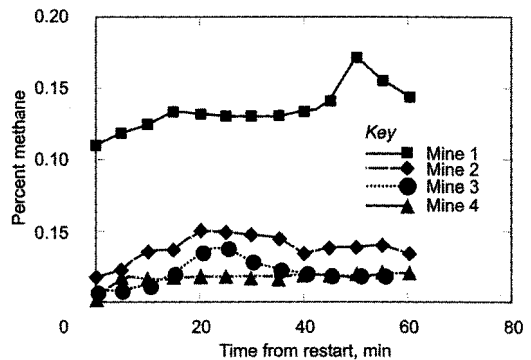
Figure 3. Methane concentrations in fan exhaust after restart.
