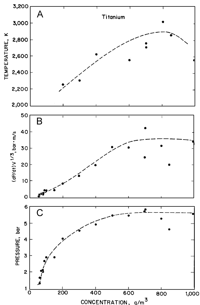
Fig. 7. Explosibility data for titanium dust.
