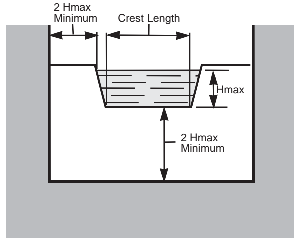
Trapezoidal (Cipolletti) Sharp-Crested Weir
