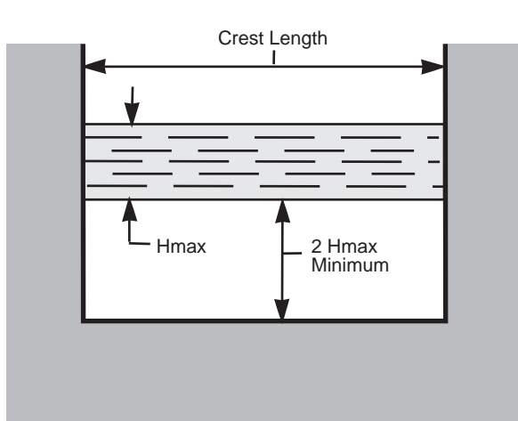
Suppressed (Without End Contractions) Rectangular Weir
