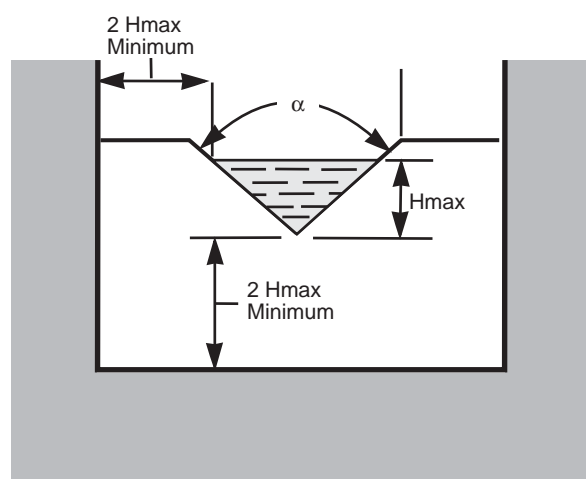
V-Notch (Triangular) Sharp-Crested Weir
