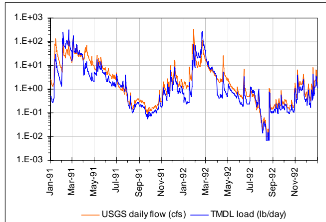
Figure 13. Estimated daily phosphorus loads.
