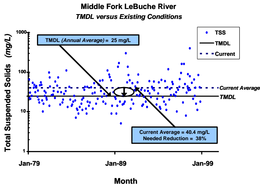
Figure 25. Example of a concentration-based TMDL.
