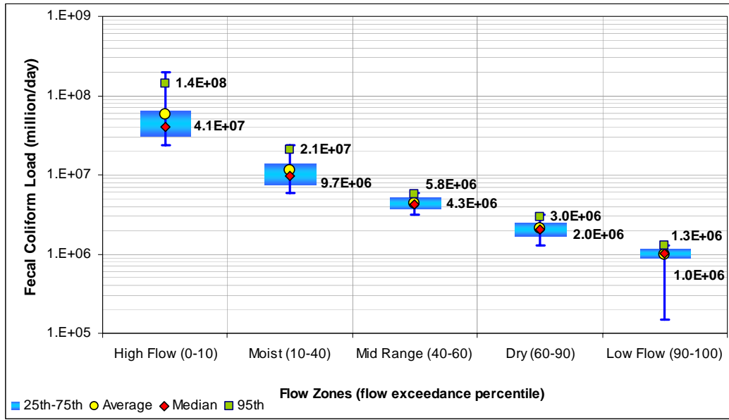
Figure 10. Daily load expressions by flow category.
