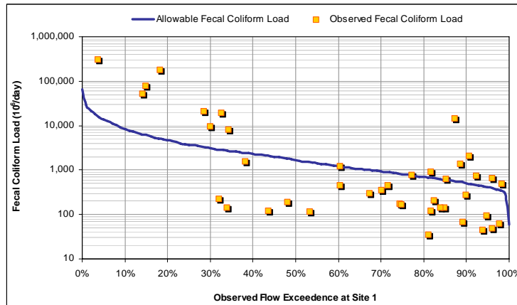
Figure 19. Load duration analysis for fecal coliform in Carter Creek.
