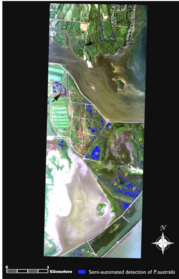
Figure 36. Results of a Spectral Angle Mapper (supervised) classification, indicating likely areas of relatively homogeneous stands of Phragmites australis (solid blue), using PROBE-1™ data and field-based ecological data. Field-sampled patches of Phragmites are shown by black arrows. Areas of mapped Phragmites are overlaid on a natural-color image of Pointe Mouillee wetland complex (August 2001). Yellow “P” indicates the general location of known areas of Phragmites , validated with aerial photographs, field notes, and 2002 accuracy assessment data.
