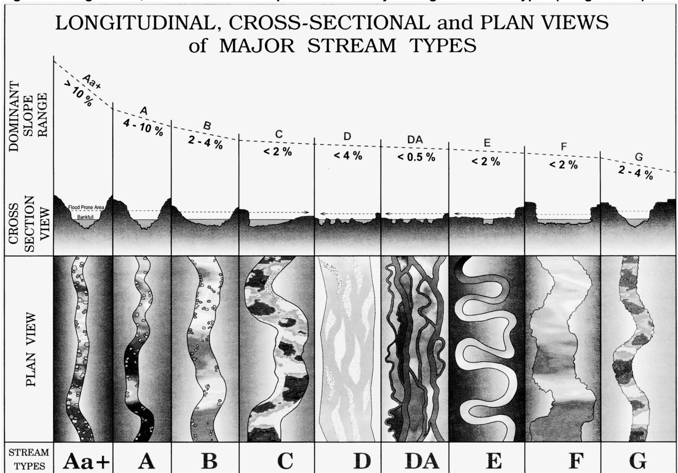
Figure 6. Longitudinal, cross-sectional and plan views of major Rosgen Channel Types (Rosgen 1996).
