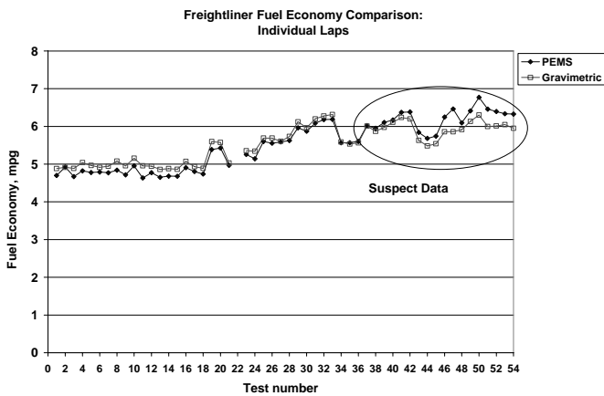
Figure 4: Comparison of fuel economy measurements for each test lap of the Freightliner control truck. There is a clear crossover in the relationship between the PEMS and gravimetric data.
