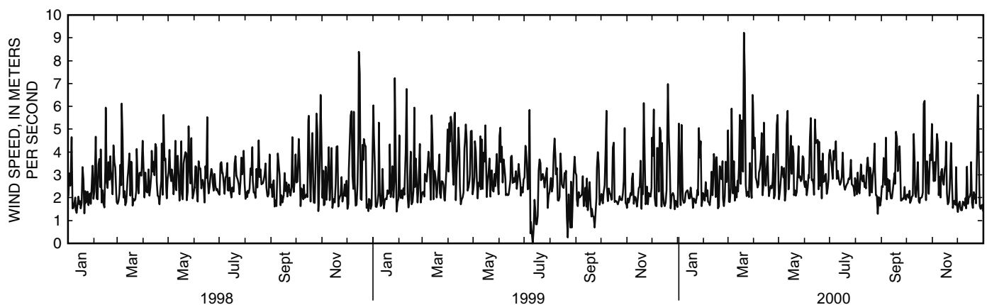
Figure 10. Daily mean wind speed at Amargosa Desert Research Site near Beatty, Nev., 1998–2000, computed from 10-second sampling intervals.
