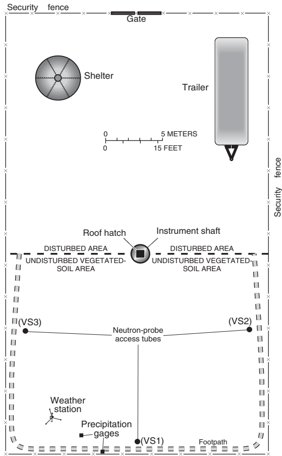
Figure 2. Fenced area of instrument shaft showing location of weather station, neutron-probe access tubes, and precipitation gages at Amargosa Desert Research Site near Beatty, Nev.
