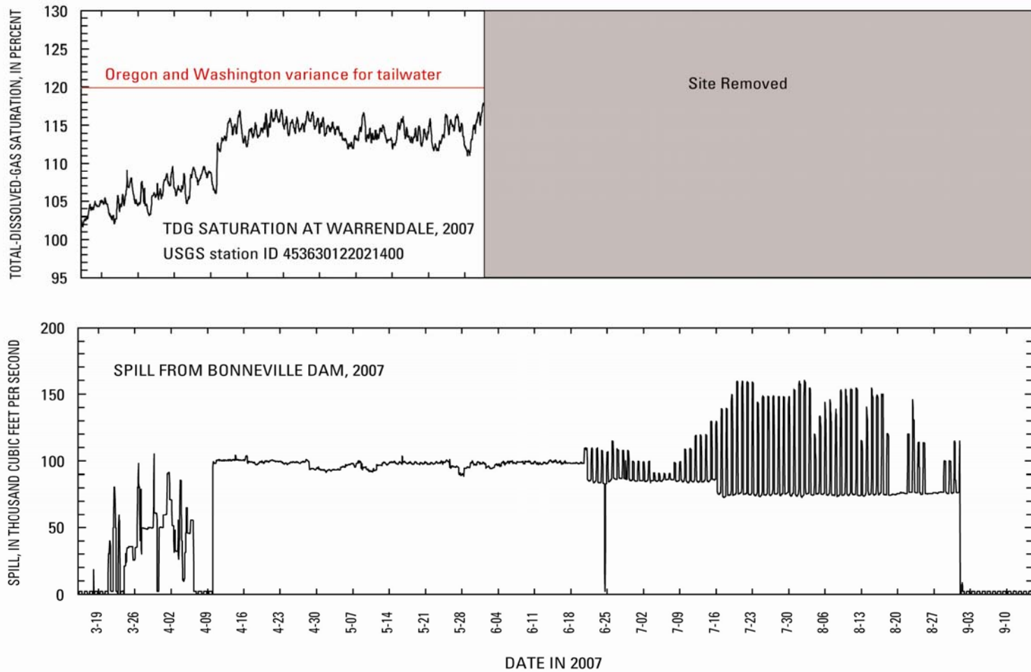
Figure 8. Total dissolved gas saturation downstream from Bonneville Dam at Warrendale and spill from Bonneville Dam, March 15 to September 15, 2007. (Date format = M-DD)
