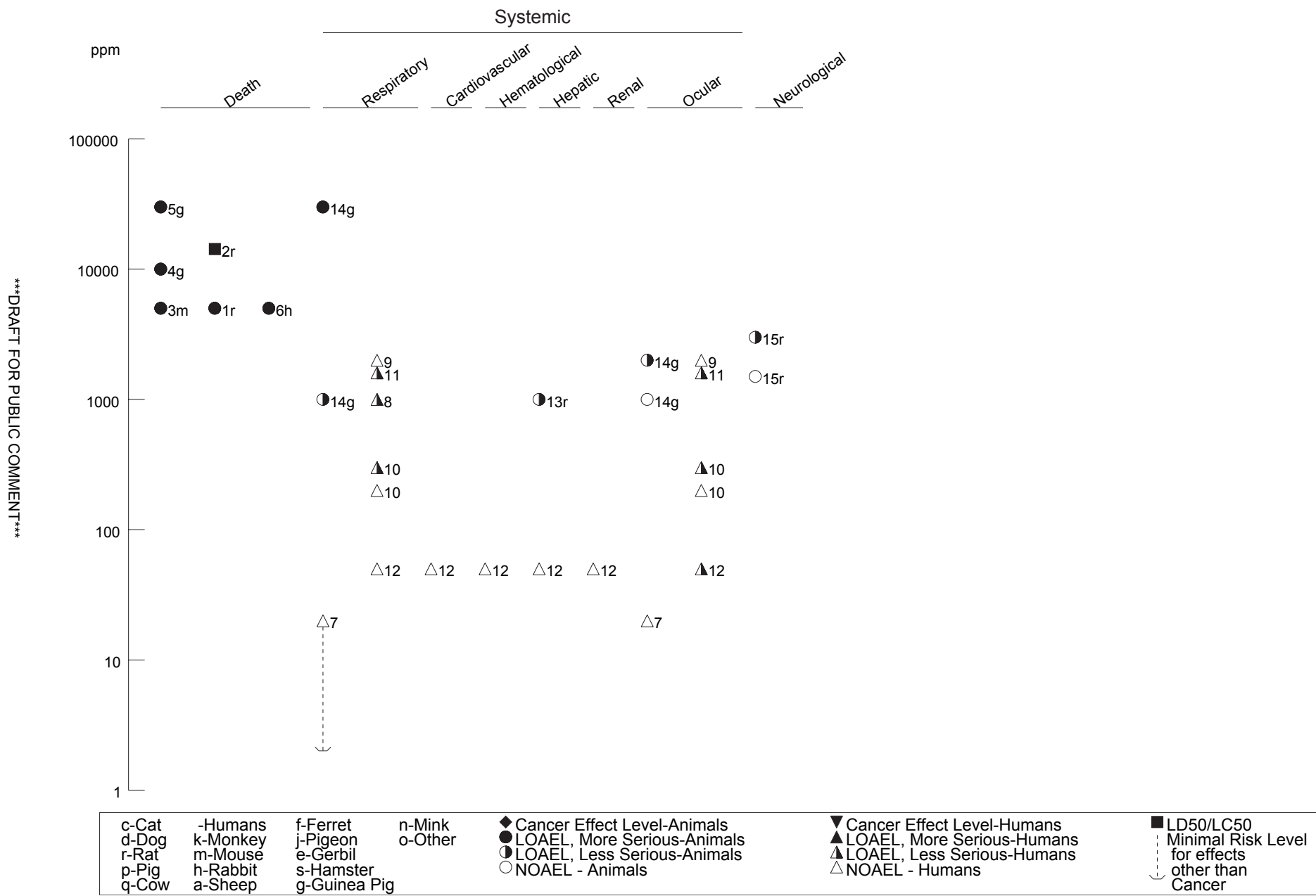
Figure 3-1 Levels of Significant Exposure to 1,4-Dioxane - Inhalation Acute (≤14 days)
