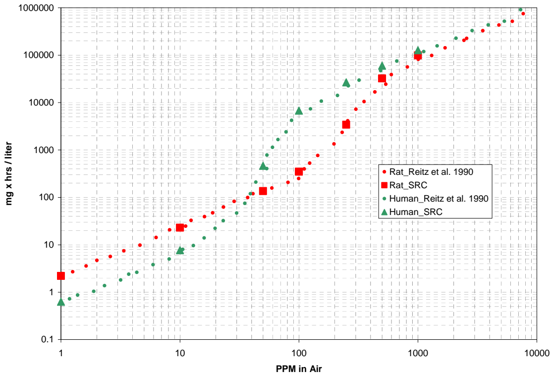
Figure B-1. Comparison of Model Output Reported in Reitz et al. (1990, Figure 5a) and from SRC Version of the Reitz et al. (1990) 1,4-Dioxane Model (Inhalation)
