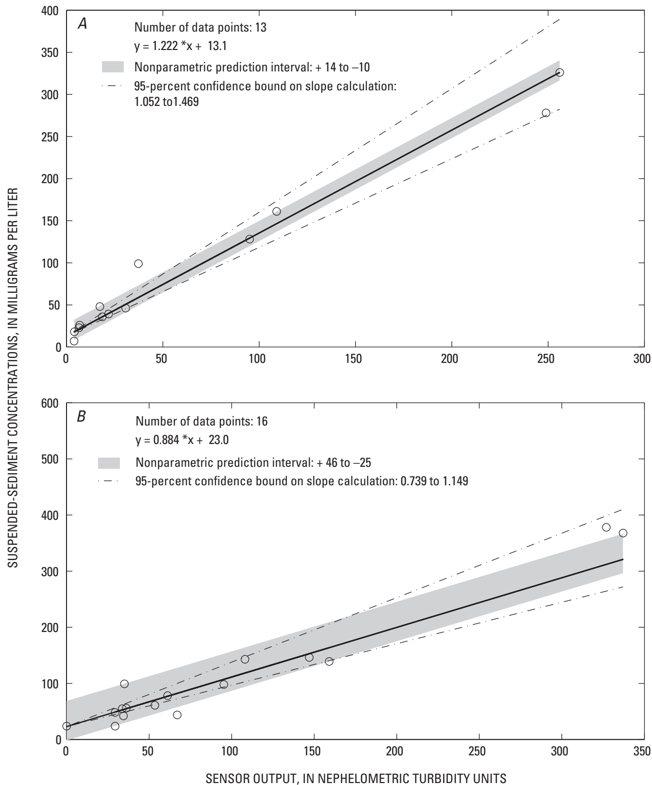
Figure 7. Calibration of mid-depth (A) and near-bottom (B) optical backscatterance sensors at Carquinez Bridge, San Pablo Bay, California, water year 2000.
