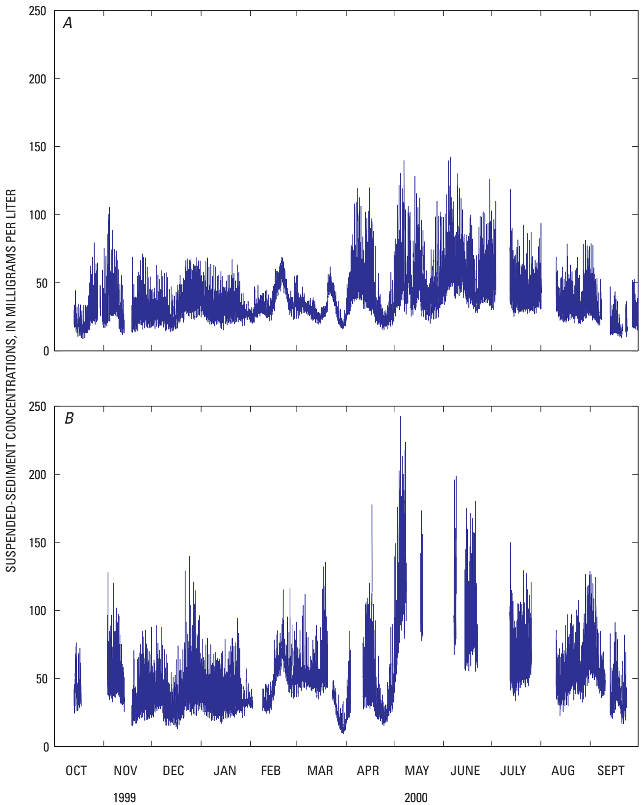
Figure 6. Time series of near-surface (A) and near-bottom (B) suspended-sediment concentrations calculated from sensor readings at Mallard Island, Suisun Bay, California, water year 2000.
