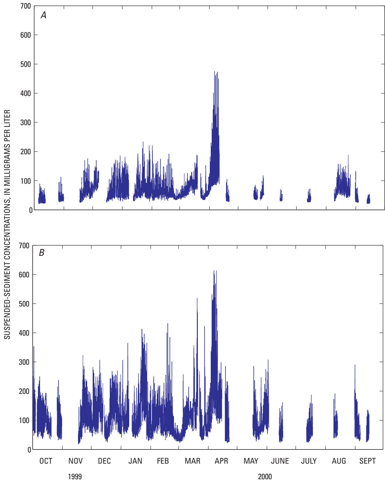
Figure 20. Time series of mid-depth (A) and near-bottom (B) suspended-sediment concentrations calculated from sensor readings at Dumbarton Bridge, South San Francisco Bay, California, water year 2000.
