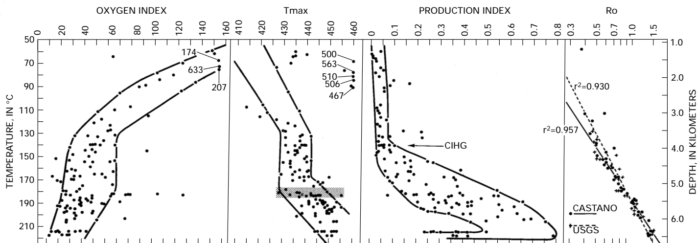
Figure 13. Plot of R_o and ROCK-EVAL oxygen-indices, T_{max} , and production indices, versus burial temperature in ^{\circ}\text{C} and depth in kilometers for siltstones and shales from six wellbores in the Paloma field, Southern San Joaquin Valley Basin. Trends defined by solid lines are discussed in the text, as is the stippled band in the T_{max} plot. Numbers at the top-right of the T_{max} and oxygen indices plots are values for the respective samples which are off the scale. Crosses and solid line in the R_o plot are U.S. Geological Survey data, dots and dashed line are R_o data from Hood and Castaño (1974). Correlation coefficients versus depth ( r^2 ) are shown for both data sets. "CIHG" in the production index plot is the commencement of intense HC generation by that plot.
