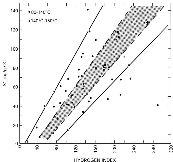
Figure 4. Cross plot of TOC-normalized ROCK-EVAL S_1 peak values ( S_1 mg/g OC) versus hydrogen index for Apex-1 shales and silts with burial temperatures of 80° to 150°C. Samples from 80° to 139.9°C are shown by dots and are largely enclosed by the solid lines. Samples from 140.0° to 150.0° are shown by crosses and are largely enclosed by the dashed lines and stippling.
