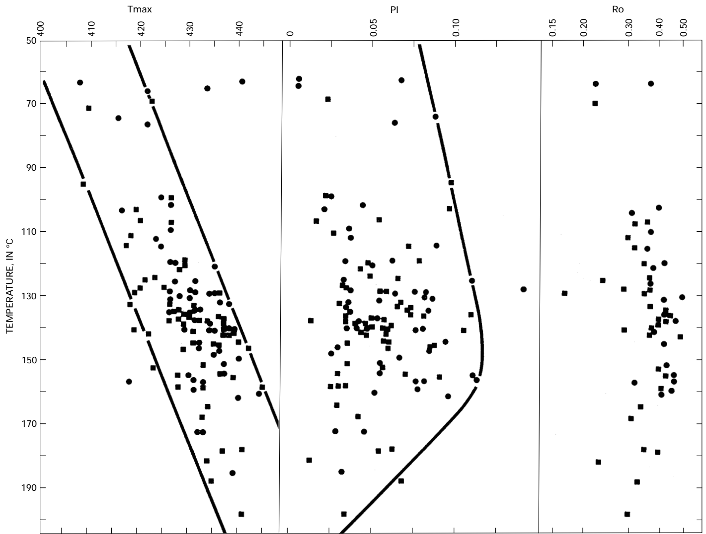
Figure 15. Plot of R_o and ROCK-EVAL T_{max} and production index (PI) values, versus burial temperature in ^{\circ}\text{C} for siltstones and shales with hydrogen-indices of 300 and greater from the Los Angeles and Ventura Basins. Trends defined by solid lines are discussed in text. Dots are samples with HI values of 300 to 400, squares are samples with HI values of 400 or above.
