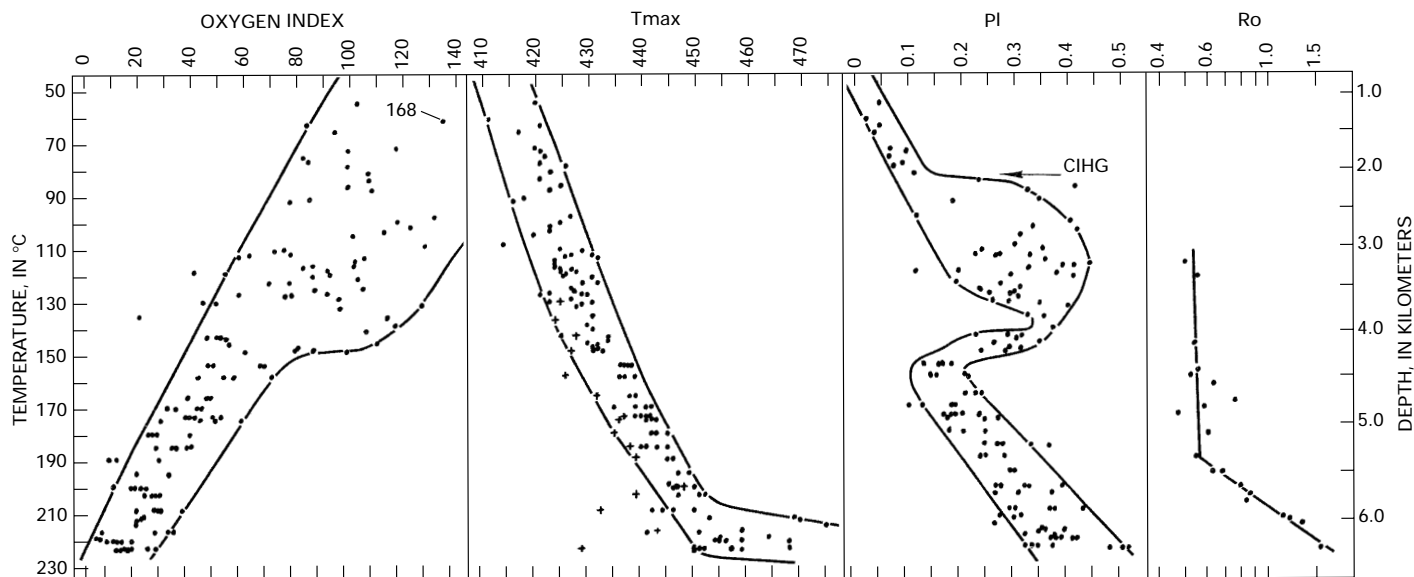
Figure 3. Plot of ROCK-EVAL oxygen index ( S_3 mg/g OC), T_{max} , production index (PI) values; and R_o versus burial temperature in °C and burial depth in kilometers for siltstones and shales from the Apex-1 wellbore. Depth axis changes scale because of a dog-leg in the geothermal gradient (table 2). Trends defined by solid lines discussed in text. Crosses in the T_{max} plot are low-TOC siltstones. "CIHG" in the PI plot is the commencement of intense HC generation as indicated by that measurement. The number 168 in the oxygen-index plot refers to a sample point with an offscale value of 168.
