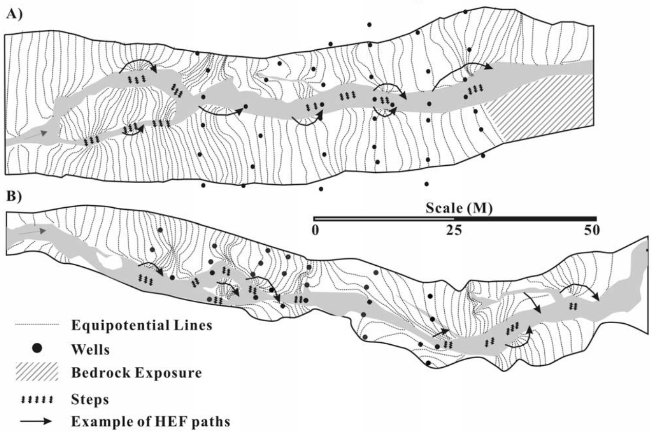
Figure 2. Site maps of (a) the WS01 study site and (b) the WS03 site. Water table elevations are predicted from MODFLOW simulations and shown with equipotential lines (0.1 m interval).
