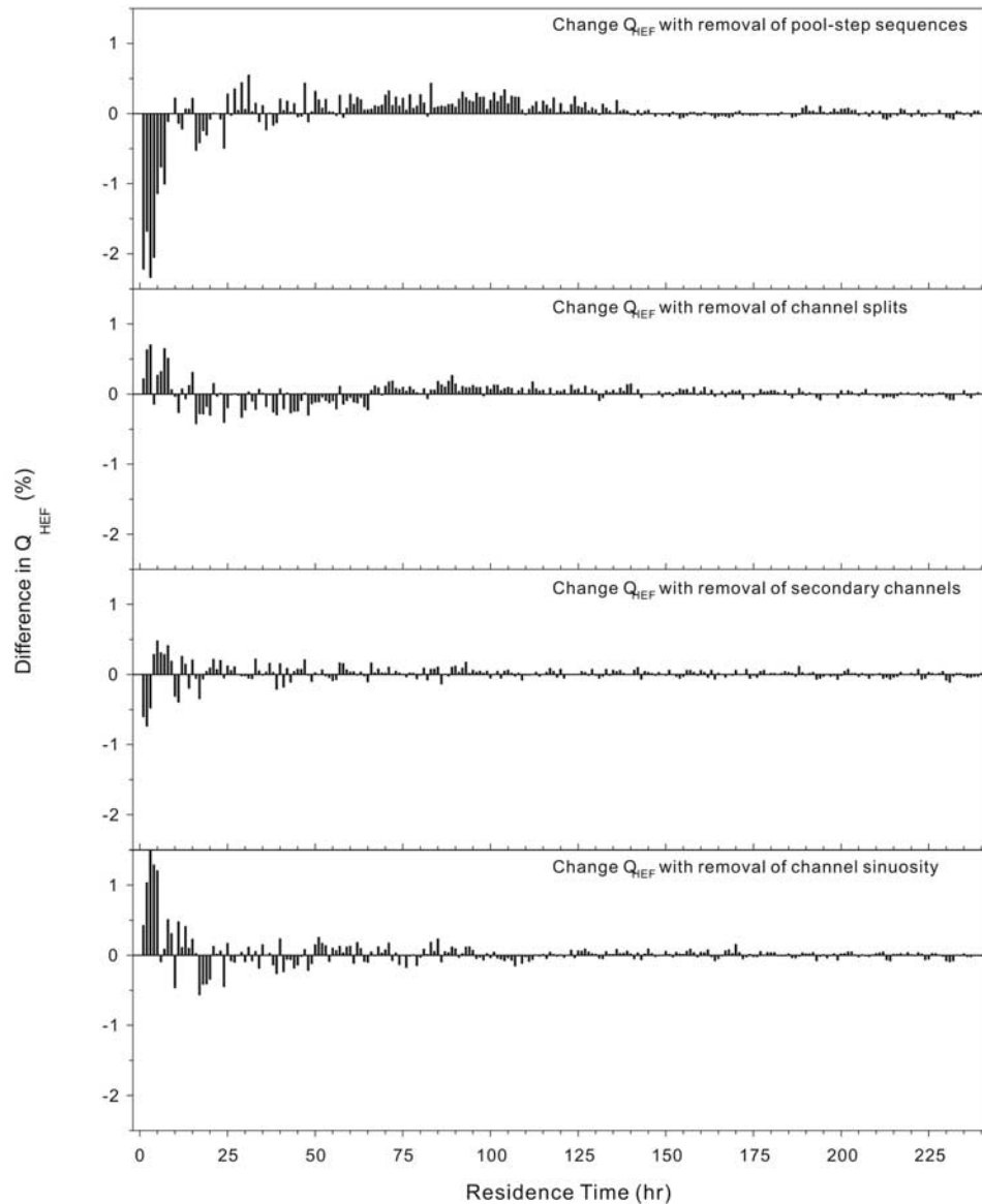
Figure 7. Changes in residence time distributions ( HEF_{RT} ) following the removal of (a) pool-step sequences, (b) channel splits, (c) secondary channels, and (d) channel sinuosity from MODFLOW simulations of the WS01 site. Negative values denote a decrease in the frequency of exchange flows with a given residence time, relative to that predicted from the original, best-fit model simulation.
