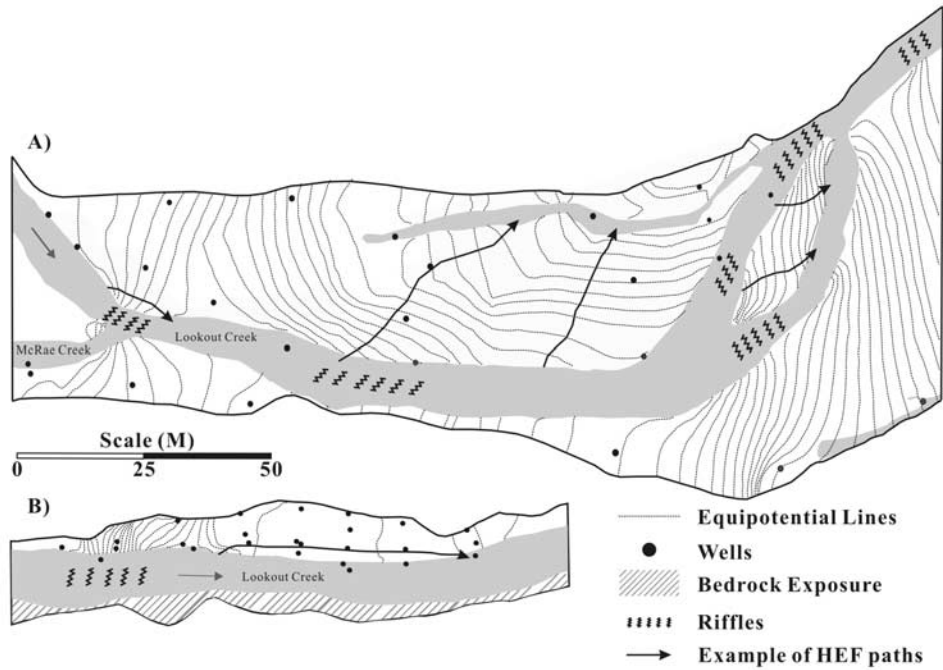
Figure 1. Site maps of (a) the Middle Lookout Creek study site and (b) the Bedrock-constrained site. Water table elevations are predicted from MODFLOW simulations and shown as equipotential lines (0.1 m interval).
