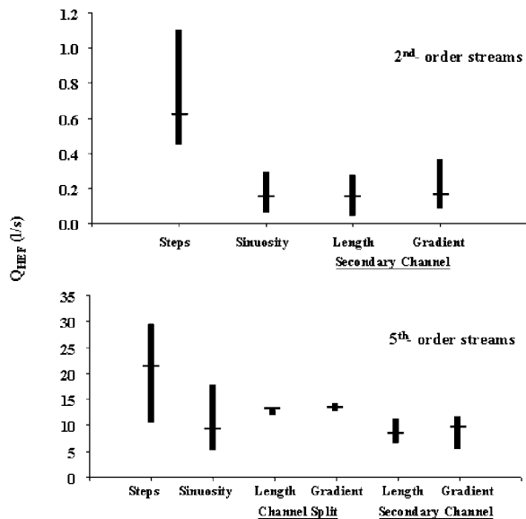
Figure 9. Sensitivity of hyporheic exchange flows ( Q_{HEF} ) to the size and number of pool-step or pool-riffle sequences, amount of channel sinuosity, the length and cross-island-bar gradients of channel splits, and length and cross-valley gradients of secondary channels predicted from simplified MODFLOW simulations of (a) the WS01 site and (b) the Middle Lookout Creek site. The maximum and minimum expression of each type of morphologic feature was determined from stream surveys.
