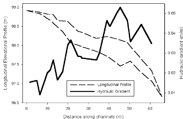
Figure 3. Longitudinal profiles of stream water elevations for the right and left stream channels at the channel split in the middle Lookout Creek study site. Bold line shows head gradient, through the island gravel bar separating the two channels.
