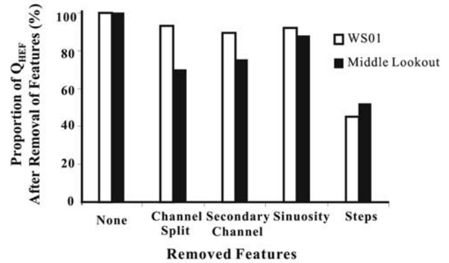
Figure 5. Comparison of predicted changes in hyporheic exchange flow ( Q_{HEF} in l/s) following the removal of classes of channel morphologic features from MODFLOW simulations for WS01 and Middle Lookout Creek. Changes in Q_{HEF} are expressed as a percentage from the original, best-fit model simulation.
