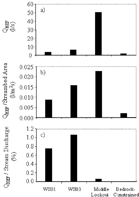
Figure 4. Amount of hyporheic exchange flow predicted from MODFLOW simulations of each study site, (a) normalized to 100-m channel length ( Q_{HEF} ), (b) normalized to streambed area ( Q_{HEF}/A ), and (c) normalized to stream discharge ( Q_{HEF}/Q ).
