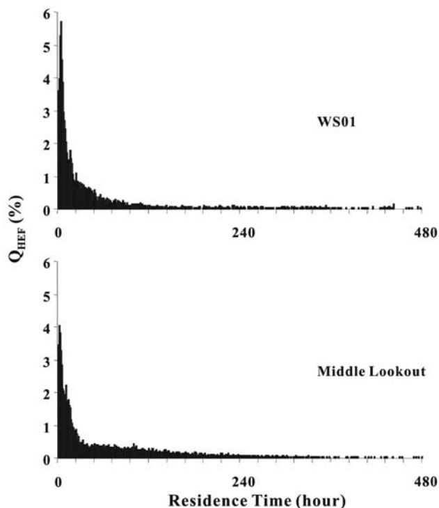
Figure 6. Residence time distributions of hyporheic exchange flows ( HEF_{RT} ) estimated using the particle-tracking routine in MODPATH, for (a) WS01 and for (b) Middle Lookout Creek. Residence times are shown as a percentage of the total, to facilitate comparisons between sites.
