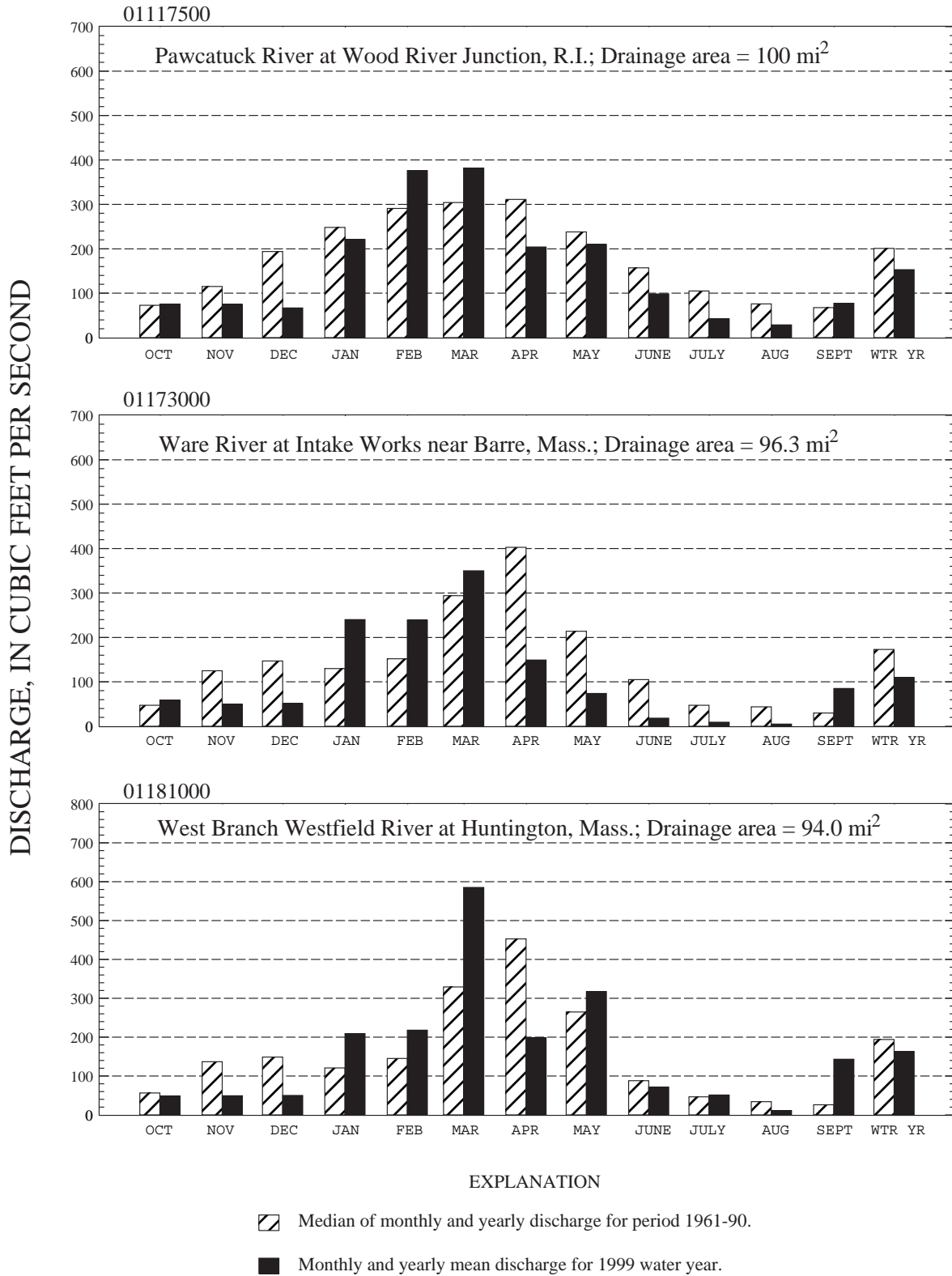
Figure 4. Comparison of discharge at three long-term index stations during the 1999 water year with median discharge for 1961-90.
