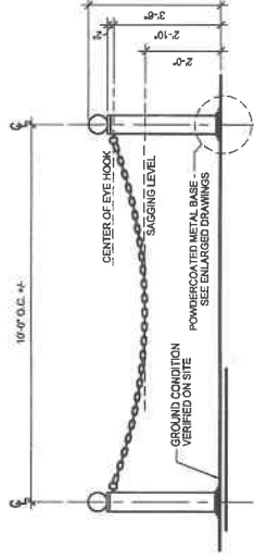
TYPICAL MOVEABLE METAL BOLLARD ON LAWN / ON PAVING - SECTION / ELEVATION 1/2" = 1'-0"
