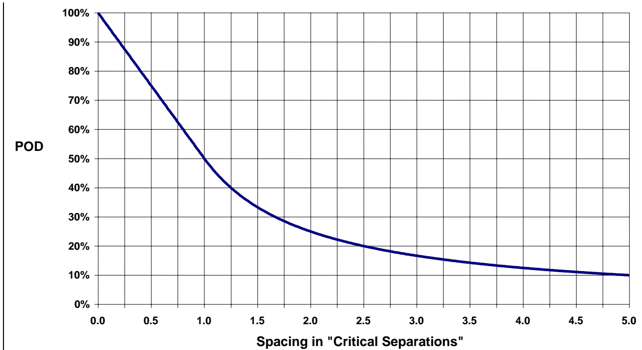
Figure 3-3. POD versus Spacing in "Critical Separations" (Perkins, 1989).
