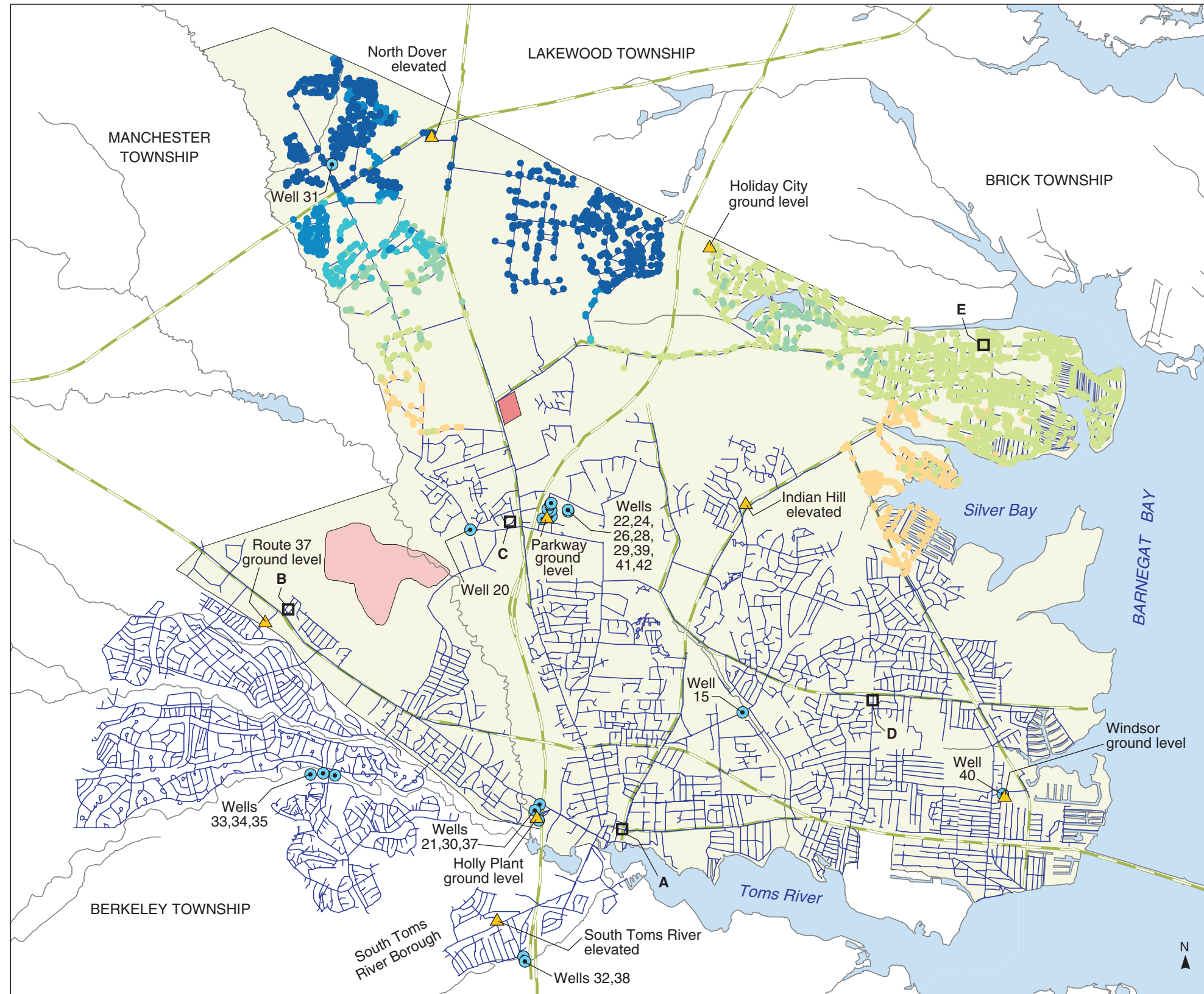
PLATE 152. AREAL DISTRIBUTION OF SIMULATED PROPORTIONATE CONTRIBUTION OF WATER FROM THE ROUTE 70 WELL (31) TO LOCATIONS IN THE DOVER TOWNSHIP AREA, NEW JERSEY, OCTOBER 1996 CONDITIONS By Morris L. Maslia, Jason B. Sautner, Mustafa M. Aral, Richard E. Gillig, Juan J. Reyes, and Robert C. Williams
