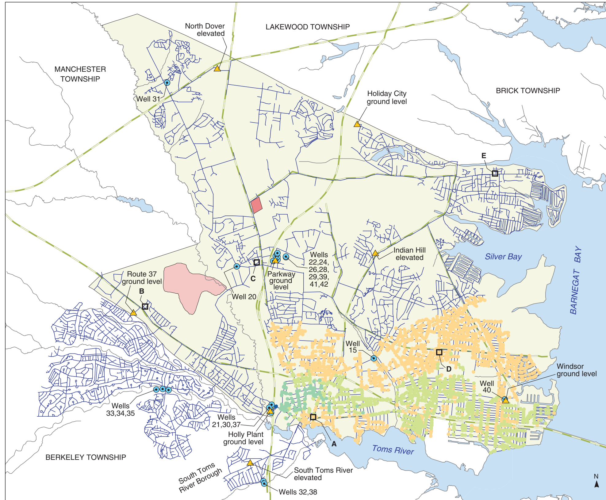
PLATE 149. AREAL DISTRIBUTION OF SIMULATED PROPORTIONATE CONTRIBUTION OF WATER FROM THE HOLLY WELL (30) TO LOCATIONS IN THE DOVER TOWNSHIP AREA, NEW JERSEY, OCTOBER 1996 CONDITIONS
