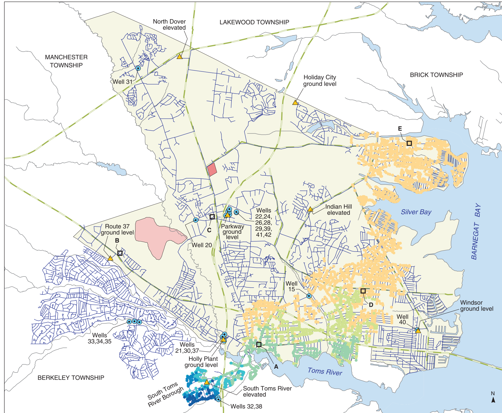
PLATE 144. AREAL DISTRIBUTION OF SIMULATED PROPORTIONATE CONTRIBUTION OF WATER FROM THE SOUTH TOMS RIVER WELLS (32, 38) TO LOCATIONS IN THE DOVER TOWNSHIP AREA, NEW JERSEY, JUNE 1996 CONDITIONS By Morris L. Maslia, Jason B. Sautner, Mustafa M. Aral, Richard E. Gillig, Juan J. Reyes, and Robert C. Williams
