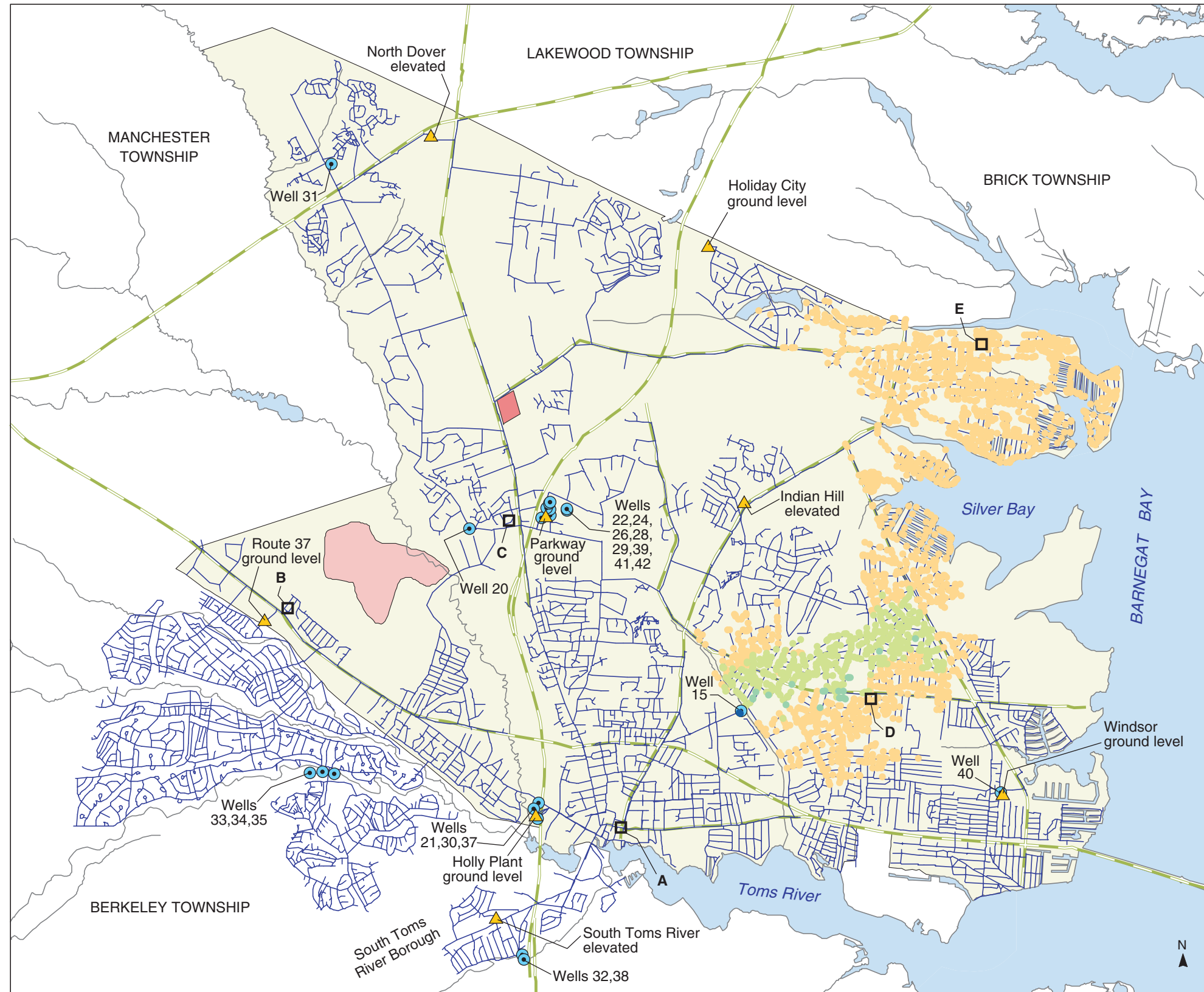
PLATE 143. AREAL DISTRIBUTION OF SIMULATED PROPORTIONATE CONTRIBUTION OF WATER FROM THE BROOKSIDE WELL (15) TO LOCATIONS IN THE DOVER TOWNSHIP AREA, NEW JERSEY, JUNE 1996 CONDITIONS
