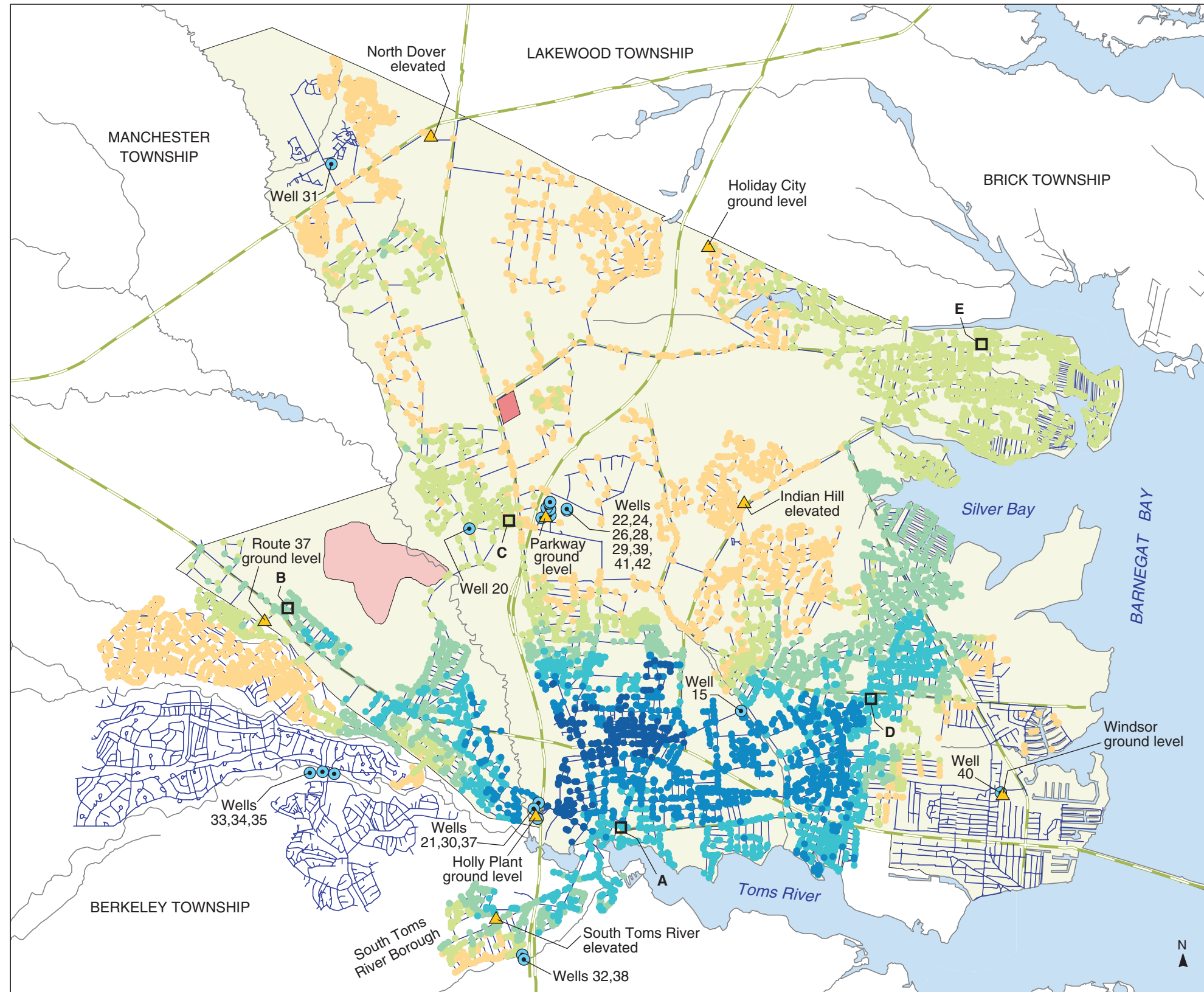
PLATE 142. AREAL DISTRIBUTION OF SIMULATED PROPORTIONATE CONTRIBUTION OF WATER FROM THE HOLLY WELL (30) TO LOCATIONS IN THE DOVER TOWNSHIP AREA, NEW JERSEY, JUNE 1996 CONDITIONS By Morris L. Maslia, Jason B. Sautner, Mustafa M. Aral, Richard E. Gillig, Juan J. Reyes, and Robert C. Williams
