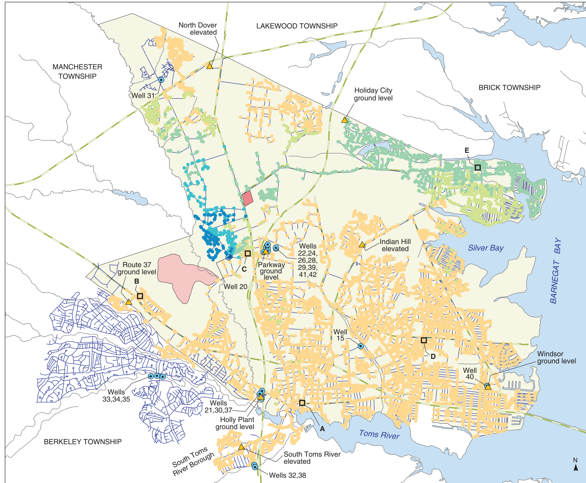
PLATE 138. AREAL DISTRIBUTION OF SIMULATED PROPORTIONATE CONTRIBUTION OF WATER FROM THE INDIAN HEAD WELL (20) TO LOCATIONS IN THE DOVER TOWNSHIP AREA, NEW JERSEY, FEBRUARY 1996 CONDITIONS By Morris L. Maslia, Jason B. Sautner, Mustafa M. Aral, Richard E. Gillig, Juan J. Reyes, and Robert C. Williams
