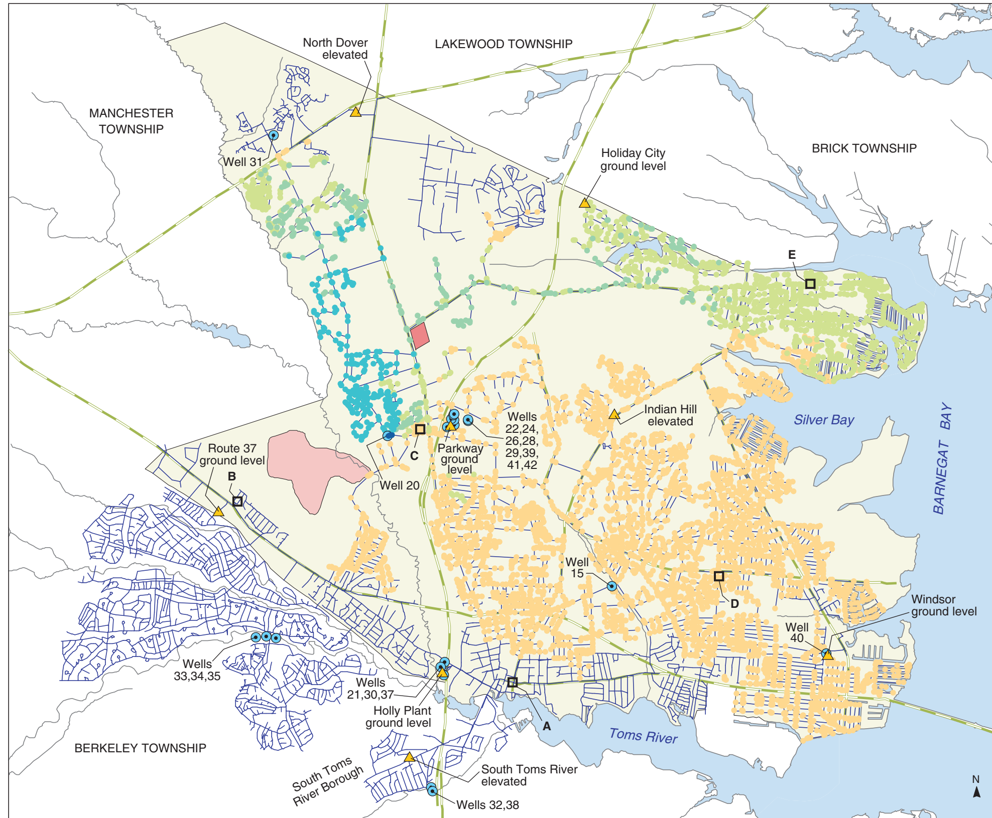
PLATE 132. AREAL DISTRIBUTION OF SIMULATED PROPORTIONATE CONTRIBUTION OF WATER FROM THE INDIAN HEAD WELL (20) TO LOCATIONS IN THE DOVER TOWNSHIP AREA, NEW JERSEY, OCTOBER 1995 CONDITIONS By Morris L. Maslia, Jason B. Sautner, Mustafa M. Aral, Richard E. Gillig, Juan J. Reyes, and Robert C. Williams
