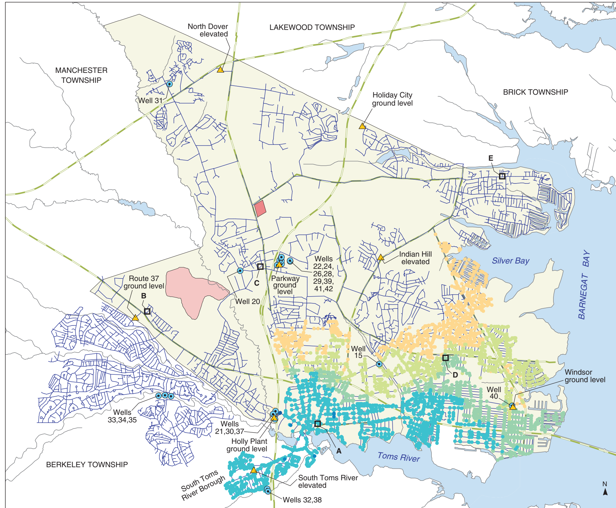
PLATE 131. AREAL DISTRIBUTION OF SIMULATED PROPORTIONATE CONTRIBUTION OF WATER FROM THE HOLLY WELL (30) TO LOCATIONS IN THE DOVER TOWNSHIP AREA, NEW JERSEY, OCTOBER 1995 CONDITIONS
