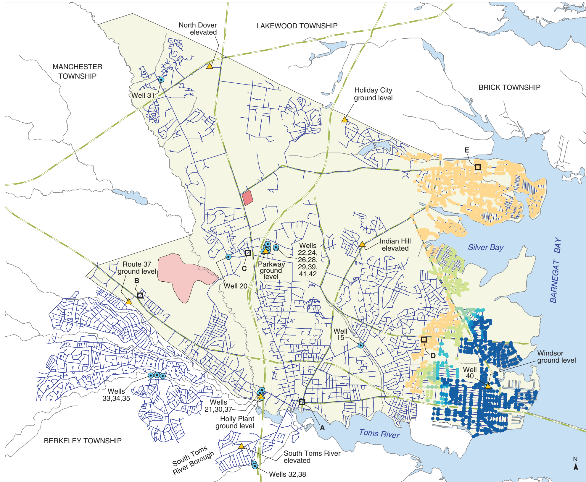
PLATE 130. AREAL DISTRIBUTION OF SIMULATED PROPORTIONATE CONTRIBUTION OF WATER FROM THE WINDSOR WELL (40) TO LOCATIONS IN THE DOVER TOWNSHIP AREA, NEW JERSEY, AUGUST 1995 CONDITIONS By Morris L. Maslia, Jason B. Sautner, Mustafa M. Aral, Richard E. Gillig, Juan J. Reyes, and Robert C. Williams
